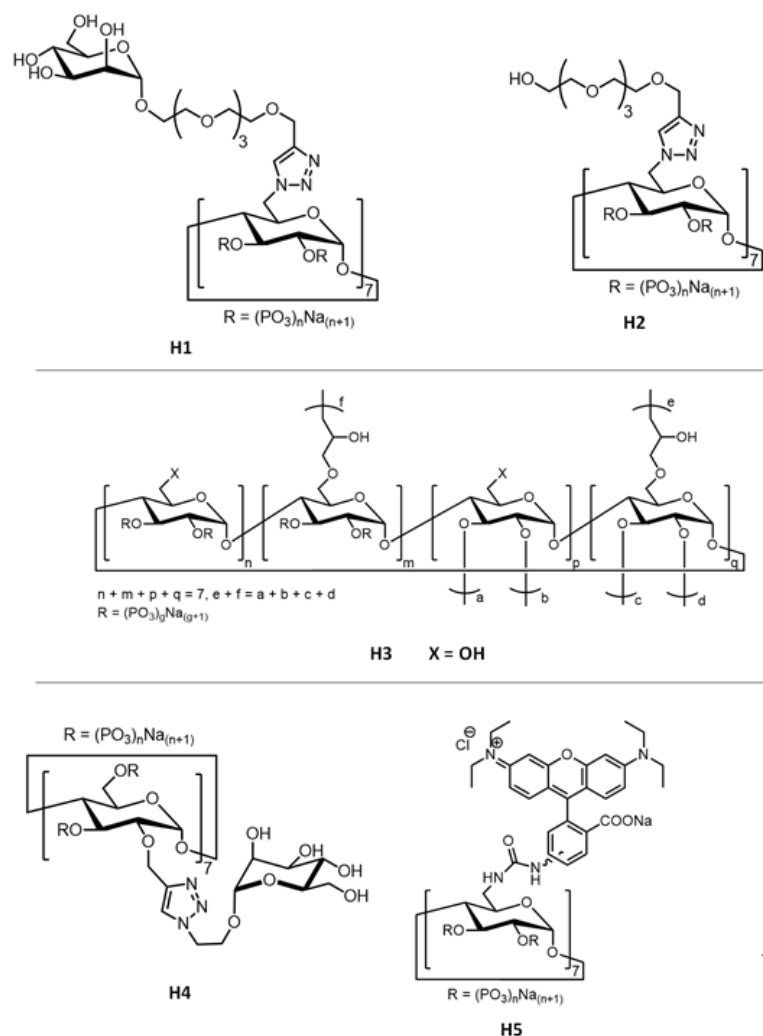
Scheme 1 Structural illustrations of H1 — H5 and L1 .
