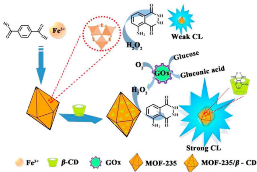
Figure 4. Proposed chemiluminescence (CL) mechanism of the luminol- \text{H}_2\text{O}_2 system by MOF-235/ \beta\text{-CD} s hybrid materials. MOF-235 is generated by the coordination reaction between \text{Fe}^{\text{III}} and terephthalic acid (top left), and further functionalized with \beta\text{-CD} . The intermediate of luminol is supposed to be hosted by the cavity of \beta\text{-CD} (right) during the oxidation reaction of glucose with glucose oxidase (GOx). Reproduced from Reference [9] with permission from Elsevier B.V. Copyright 2018.
