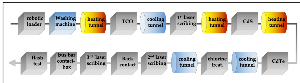
Schematic of the in-line machine for the production of large PV modules based on CdTe technology.
