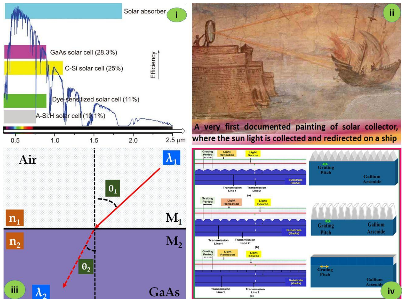
Figure A: This figure is reproduced using the original sources published in References [1][8][9] ; (i) the relative difference in efficiency of a small-area various types of solar cells together with their light absorption range, (ii) a concept of manipulating and guiding the light into a desired direction, (iii) relation in between media dependent angle of incidence and reflection, and (iv) schematic diagram for different types of nano-structured media helpful to engineer the light incidence reflection and trapping inside the nano-structures.
