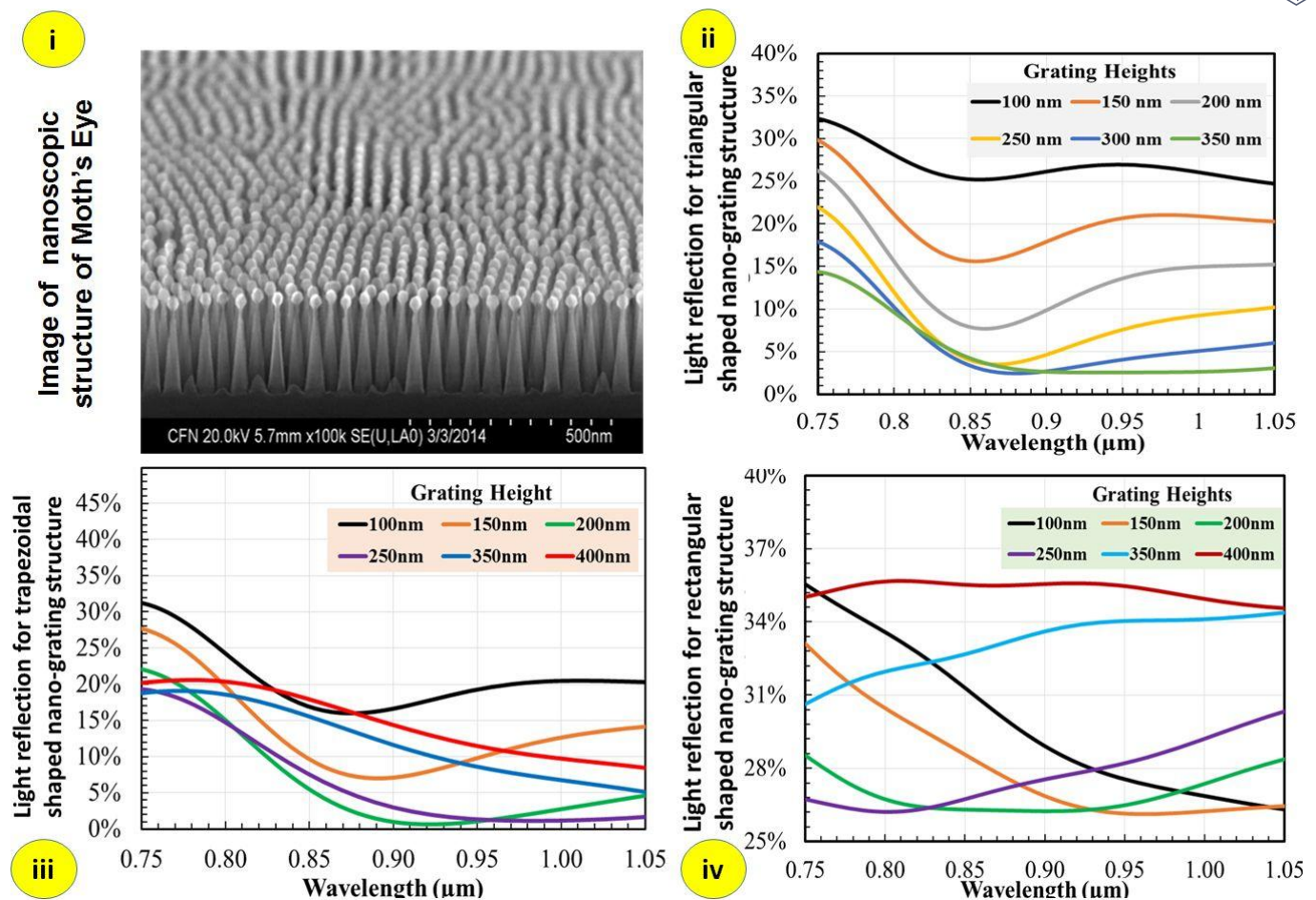
Figure B: This figure is reproduced using the original simulated results published in Reference [1] together with the image of nanoscopic structure of Moth's eye sourced out from the reference [16] ; (i) image of nanoscopic structure of Moth's eye, and (ii-iv) light reflection spectra obtained for triangular, trapezoidal and rectangular shapes of nano-gratings at different grating-height.
