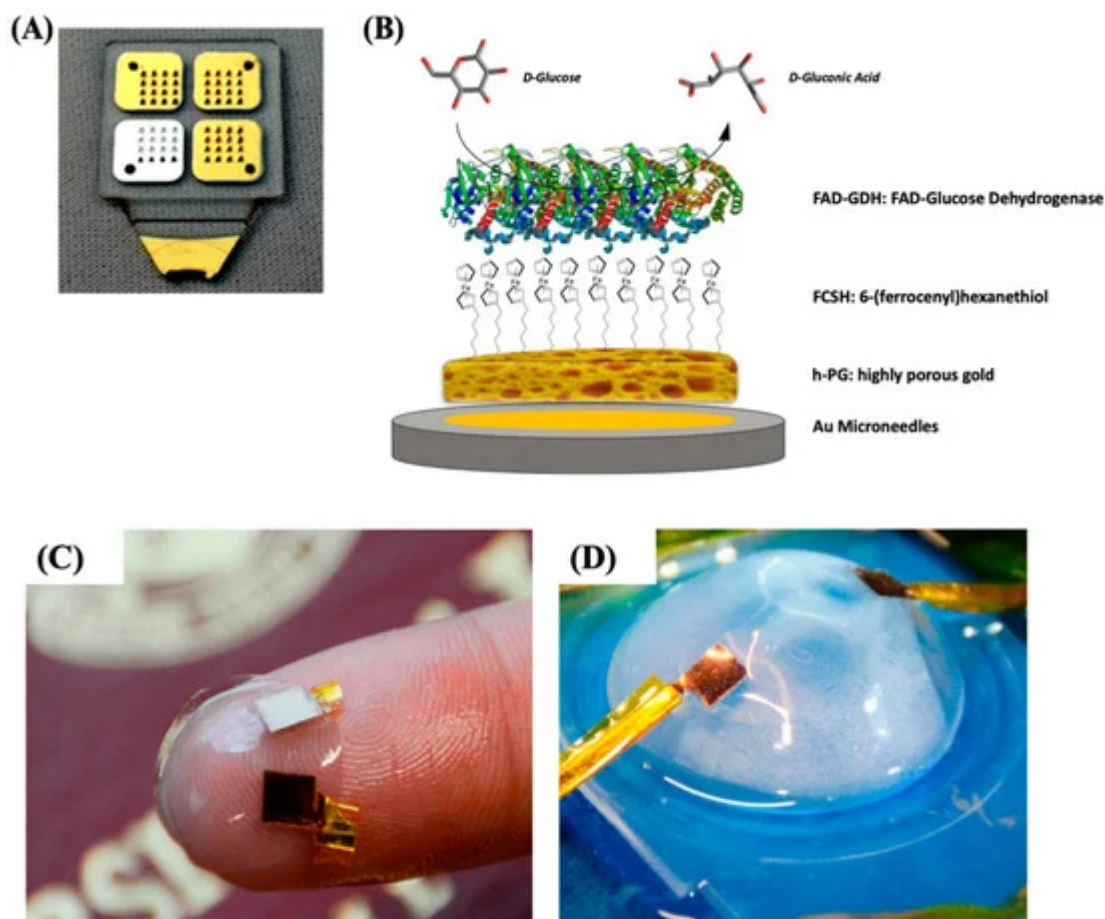
Figure 2. (A) Photo of four 4 \times 4 microneedle arrays metallized with gold and silver and (B) schematic representation of the highly porous gold (h-PG)/6-(ferrocenyl)hexanethiol (FcSH)/flavin adenine dinucleotide glucose dehydrogenase (FAD-GDH)/Au microneedle-based glucose biosensor. Photograph of the contact lens encapsulated enzymatic fuel cell (EFC; C) and testing setup (D). Figure 2A,B are reproduced with permission from [15]. Copyright MDPI, 2019. Figure 2C,D are reproduced with permission from [18]. Copyright American Chemical Society, 2018.
