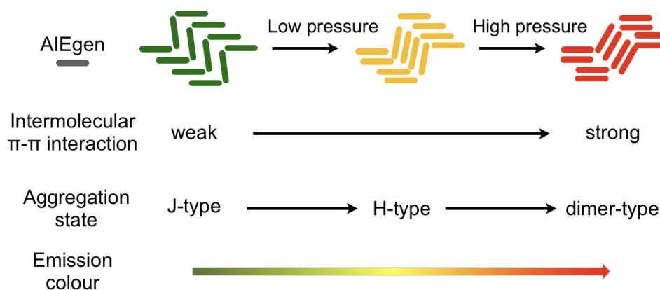
Figure 1. Schematic diagram of stacking mode and emission colour with various molecular aggregation states in a generic AIE luminogen. Adapted with permission. Copyright (2013) John Wiley and Sons.
