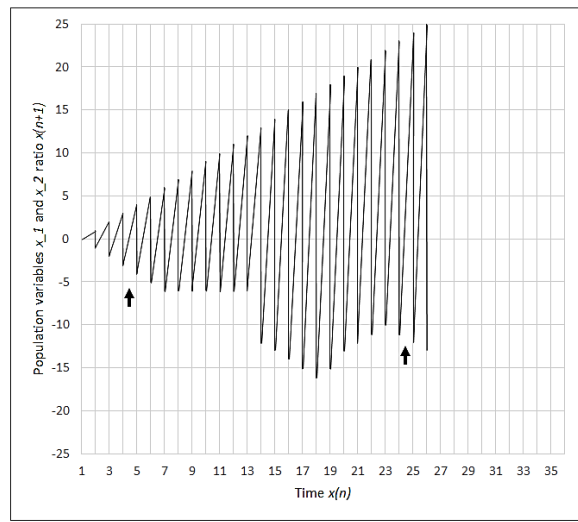
Figure 5. Time series of population variables x_1 and x_2 expressing disproportionality for population-resource ratio. The asymmetrical pattern shows recurrence at original state (indicated arrows) and time regulation equilibrium.
