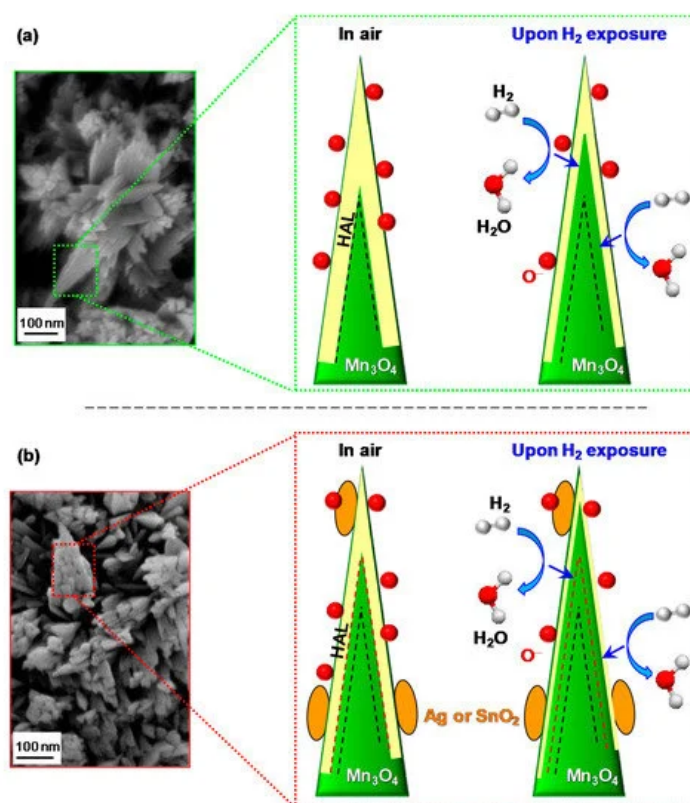
Figure 7. Schematics of the hydrogen gas sensing mechanism and corresponding hole accumulation layer (HAL) modulation for nanosystems based on: (a) bare Mn_3O_4 ; (b) functionalized Mn_3O_4 . The dashed black and red lines indicate the HAL boundaries in air in case of bare and functionalized Mn_3O_4 , respectively. Red spheres, yellow areas, and orange ovals indicate adsorbed oxygen, HAL thickness, and functionalizing agent (Ag or SnO_2 ), respectively. Blue arrows indicate electron flow due to H_2 oxidation (see reaction 4).
