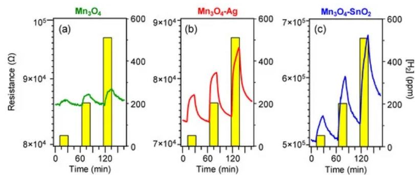
Figure 6. Dynamical responses of \text{Mn}_3\text{O}_4 (a), \text{Mn}_3\text{O}_4\text{-Ag} (b) and \text{Mn}_3\text{O}_4\text{-SnO}_2 (c) nanosystems vs. different \text{H}_2 concentrations, at a fixed working temperature of 200 °C.
