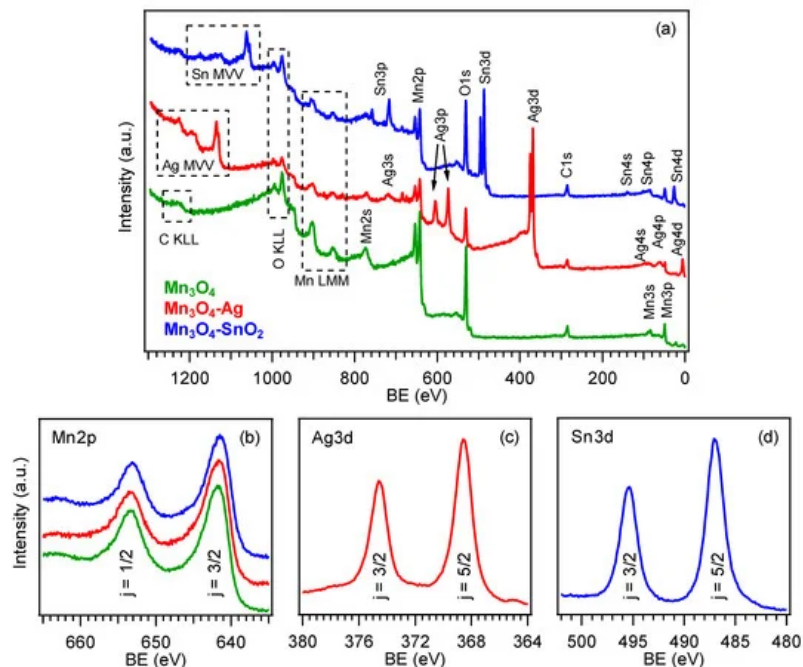
Figure 3. (a) X-ray photoelectron spectroscopy (XPS) wide-scan spectra pertaining to bare \text{Mn}_3\text{O}_4 , \text{Mn}_3\text{O}_4\text{-Ag} and \text{Mn}_3\text{O}_4\text{-SnO}_2 samples. (b) \text{Mn}2p , (c) \text{Ag}3d and (d) \text{Sn}3d photoelectron peaks. The color code is reported in panel (a).
