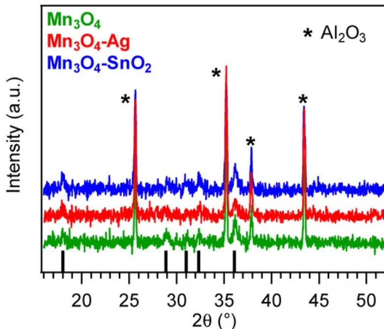
Figure 2. X-ray diffraction (XRD) patterns for bare and functionalized \text{Mn}_3\text{O}_4 nanosystems. Vertical black bars correspond to \alpha\text{-Mn}_3\text{O}_4 signals [53].
