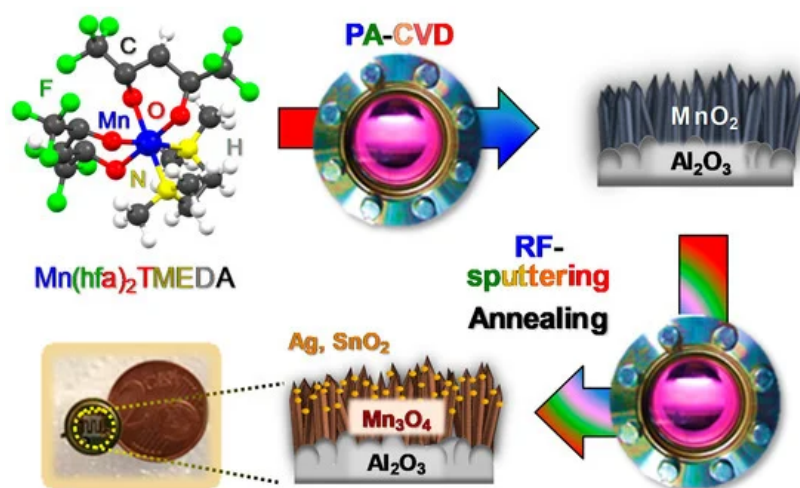
Figure 1. Scheme of the route proposed in the present study for the fabrication of \text{Mn}_3\text{O}_4 -Ag and \text{Mn}_3\text{O}_4 - \text{SnO}_2 nanomaterials.
