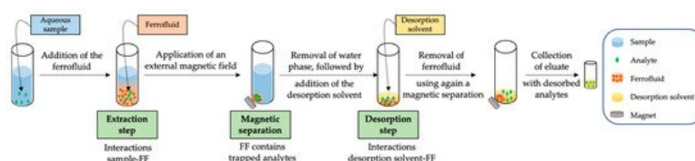
Figure 1. General scheme of the most common operational procedure followed in ferrofluid (FF)-based analytical extraction methods.
