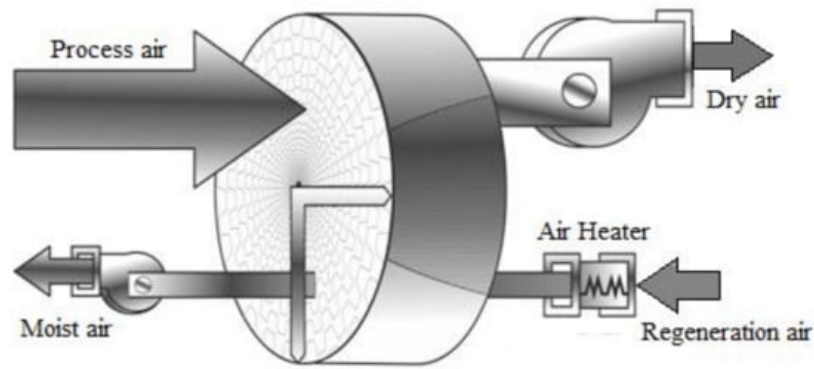
Figure 1. Rotary Desiccant Dehumidification System.
