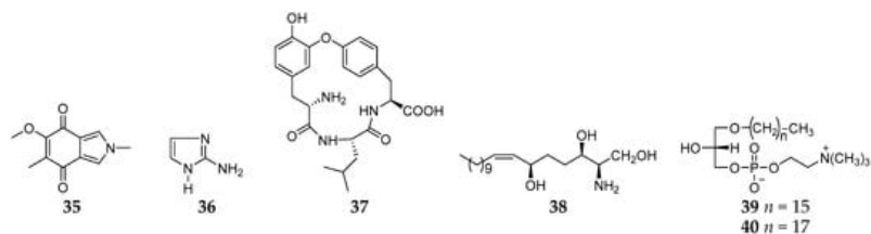
Figure 4. Other alkaloids derivatives 35–40 from the subgenus Reniera .
