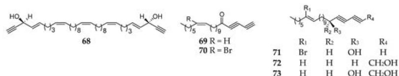
Figure 7. Aliphatic polyketides 68–73 from the subgenus Reniera .
