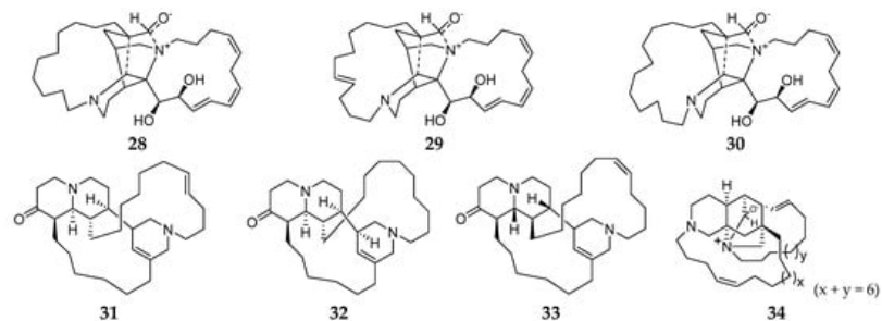
Figure 3. Macrocyclic diamines derivatives 28–34 from the subgenus Reniera .
