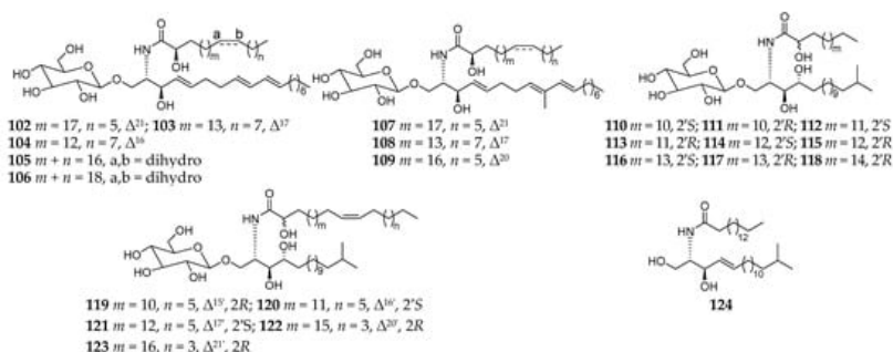
Figure 10. Cerebrosides 102–123 and ceramide 124 from the subgenus Reniera .
