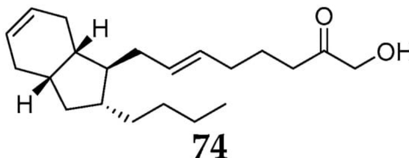
Figure 8. Other polyketide 74 from the subgenus Reniera .
