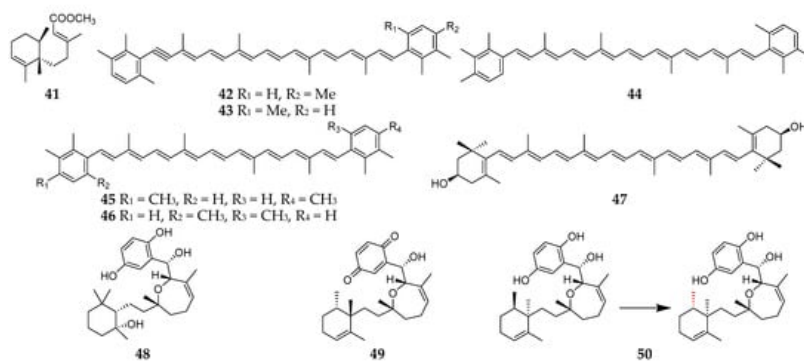
Figure 5. Terpenoids 41–50 from the subgenus Reniera .
