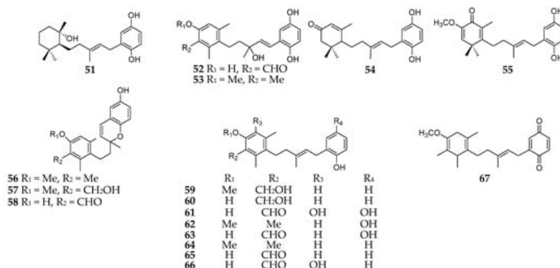
Figure 6. Aromatic polyketides derivatives 51–67 from the subgenus Reniera .
