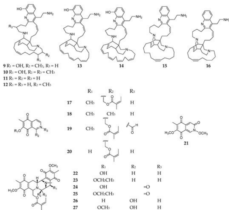
Figure 2. Quinolines and isoquinolines 9–27 from the subgenus Reniera .
