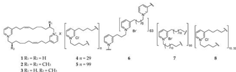
Figure 1. 3-Alkylpyridiniums 1–5 from the subgenus Reniera and their derivatives 6–8 .
