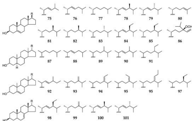
Figure 9. Sterols 75–101 from the subgenus Reniera .
