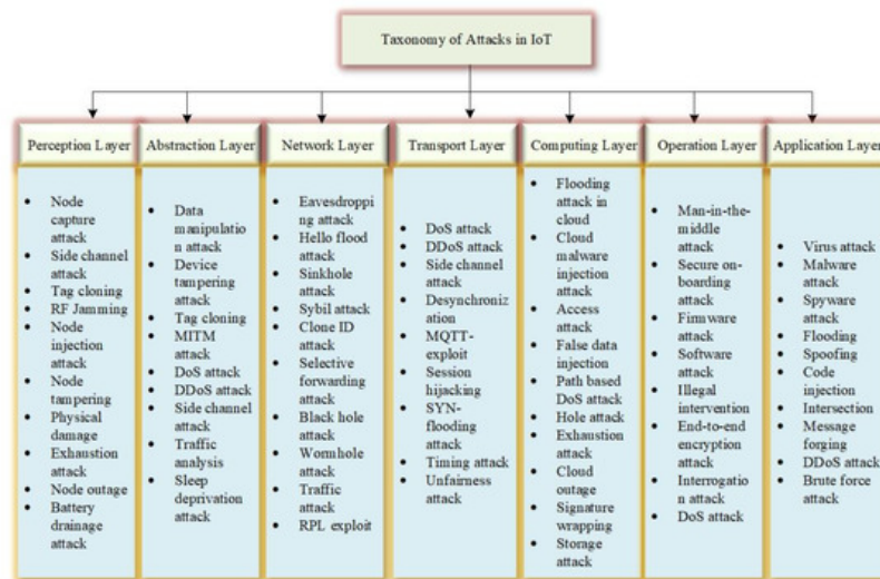
Figure 2. Taxonomy of attacks in IoT.
