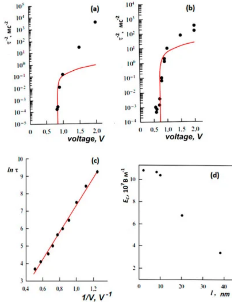
Figure 6. The dependence of the switching time \tau on the applied voltage for 8-nm-thick \text{BaTiO}_3 film [1][3][29]: (a) in the capacitor and (b) in the probe mode in an atomic force microscope (lines \tau^{-2}(V) on (a) and (b) correspond to the calculations according to formula (7)); (c) for a \text{BaTiO}_3 crystal, the line corresponds to \ln[\tau(V^{-1})] and is obtained relying on the piezo-response mode in an atomic force microscope; (d) the dependence of the coercive field on the thickness of the \text{BaTiO}_3 film. Reproduced with permission from [29]; Elsevier, 2013. The switching kinetics in these ultrathin single-crystal \text{BaTiO}_3 epitaxial laser films of 2–8 and 40 nm thickness synthesized on a \text{SrRuO}_3/\text{SrTiO}_3 substrate were studied in a \text{SrRuO}_3 –ITO capacitor using an atomic force microscope. A detailed description of the technique is presented in [30]. The distinction between proper and improper behavior is shown in Figure 5, which shows the dependence of the switching time \tau on the applied voltage V for a film of 8 nm thickness in a capacitor (Figure 6a), and under a tip of an atomic force microscope (Figure 6b). For comparison, the same dependence for a bulk \text{BaTiO}_3 single crystal of 1 mm thickness is shown in Figure 6c.
