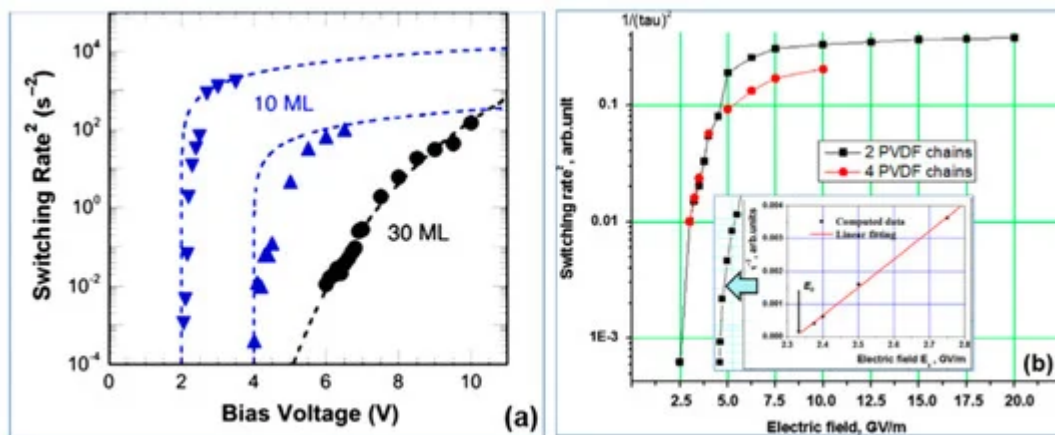
Figure 3. Switching time \tau_s for polymer ferroelectrics presented as \tau^{-2} along E in a logarithmic scale: (a) experimental data [14][15] for thin LB of P(VDF-TrFE) film of 10 ML (5 nm) with critical behavior of \tau^{-2} for E \rightarrow E_C in comparison with thick 30 ML (15 nm) films with exponential low (Reproduced with permission from [14]; AIP Publishing, 2011); (b) MD simulation run data [18][19] for PVDF models showing the critical behavior of \tau^{-2} with a change in E , which qualitatively coincides with the experimentally observed behavior; the inset shows the linear behavior of \tau^{-2} as E \rightarrow E_C and determines the critical value of E_C \sim 2.3 GV/m (Reproduced with permission from [18]; Elsevier, 2014).
