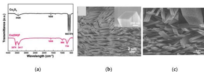
Figure 11. FTIR spectra of the Co 3 O 4 NRs: (a) before and after sintering at 450 °C; (b) SEM images of Co(OH)F NR; (c) SEM image of the rhombus-shaped Co 3 O 4 NR arrays annealed at 450 °C. Reprinted with the permission from [25].
