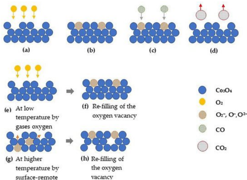
Figure 15. The schematics of proposed CO detection mechanism: (a,b) adsorption of O 2 to the Co 3 O 4 surface; (c) adsorption of CO to the Co 3 O 4 surface once it reacts with surface-near lattice oxygen; (d) the desorption of CO as CO 2 ; (e,f) oxygen vacancies are replenished by oxygen from the gas phase; (g,h) replenishment of oxygen vacancies by oxygen from the surface-remote lattice. Redrawn with the permission from [28].
