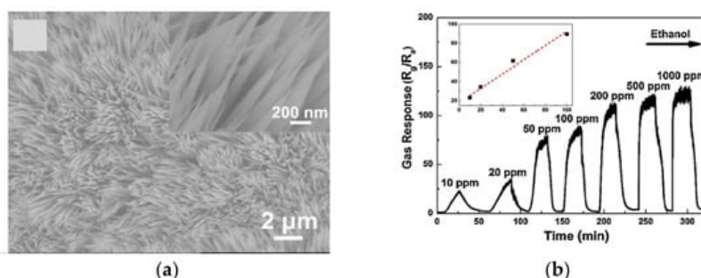
Figure 12. The SEM image of \text{Co}_3\text{O}_4 : (a) nanoneedle arrays; (b) the dynamic response and recovery plot of the \text{Co}_3\text{O}_4 toward ethanol. Reprinted with the permission from [34].
