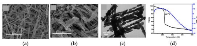
Figure 19. Morphological features of the mesoporous \text{Co}_3\text{O}_4 nanochains: (a) SEM; (b) TEM; (c) HRTEM images; (d) TG and DTA plots of cobalt carbonate hydroxide nanowire. Reprinted with the permission from [82].
