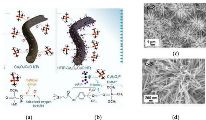
Figure 22. The schematic of DMMP-sensing mechanism: (a) \text{Co}_3\text{O}_4/\text{CuO} NTs; (b) hybrid HFIP- \text{Co}_3\text{O}_4/\text{CuO} NTs. Reprinted with the permission from [89]; (c,d) SEM micrograms of the reported NWs array. Reprinted with the permission from [22].
