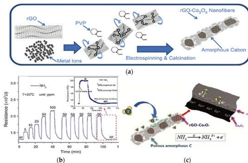
Figure 18. The schematic illustration of growth mechanism: (a) rGO- \text{Co}_3\text{O}_4 composite nanofibers; (b) dynamic response toward the \text{NH}_3 ; (c) schematic diagram of the sensing mechanism of the rGO- \text{Co}_3\text{O}_4 composite nanofibers toward ammonia at room temperature. Reprinted with the permission from [74].
