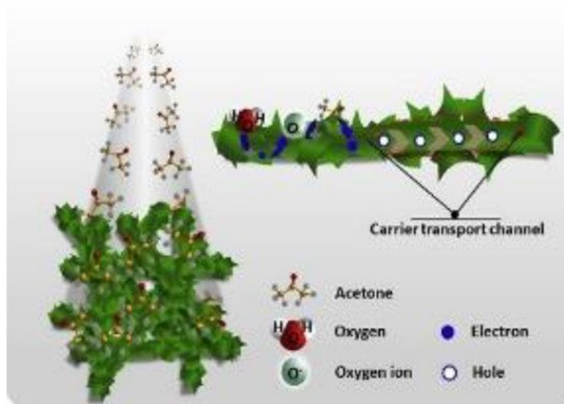
Figure 13. The illustration of sensing mechanism of C_3H_6O on Co_3O_4 . Reprinted with the permission from [52].
