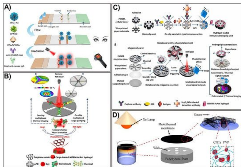
Figure 4. Schematic design of an amplified PAD signal using photothermal-based techniques. (A) Schematic representation of the \text{MnO}_2 -Au-based dual-signal immunoassay for AOX detection. Adapted with permission from Ref. [100]. (B) Principle of photothermal microfluidic pumping-based PAD fabrication. Adapted with permission from Ref. [102]. (C) The design of the clip-magazine-assembled photothermal biosensing disk for tri-mode visual quantification of prostate-specific antigen. Adapted with permission from Ref. [103]. (D) Schematic demonstration of CNT@PVP photothermal membrane-based solar steam-generation device fabrication for water desalination. Adapted with permission from Ref. [104].
