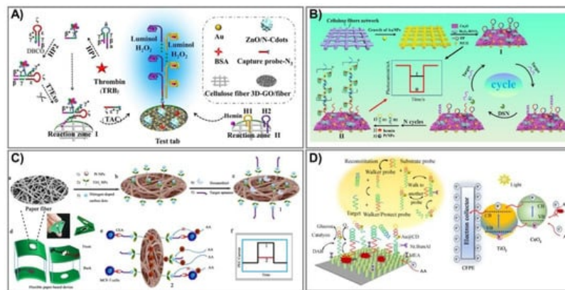
Figure 6. Photoelectrochemical paper-based analytical devices. (A) The intrinsic light Au@3D-rGO/cellulose sensor generates a photocurrent signal to detect protein in clinical biomedicine. Adapted with permission from Ref. [142]. (B) The construction process and mechanism for cathode PEC PADs shown to detect microRNA-141 by duplex-specific-nuclease (DSN) connection. Adapted with permission from Ref. [143]. (C) The PEC TiO 2 -Pt/PWE biosensor was fabricated by modification of paper with N-carbon dots/TiO 2 -Pt with a seed-mediated growth method to detect carcinoembryonic antigen (CEA). (a–c) preparation of photoelectrochemical biosensor, (d) diagram of paper-based platform, (e) detection mechanism, (f) photocurrent intensity with/without CEA. Adapted with permission from Ref. [144]. (D) An ultrasensitive PEC paper-based device to determine miRNA-141 from a two-enzyme-engineered DNA walker and a TiO 2 /CeO 2 heterojunction. Adapted with permission from Ref. [128].
