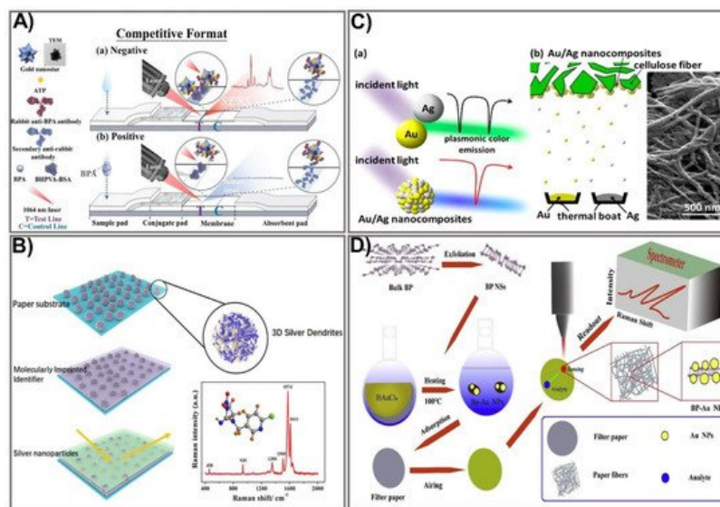
Figure 3. SERS-based signal amplification strategies for PADs. (A) The schematic principle of a gold nanostar-based SERS substrate for the sensing of biphenol A. Adapted with permission from Ref. [84]. (B) The design process for a multilayer SERS paper substrate for neonicotinoid pesticide sensing. Adapted with permission from Ref. [86]. (C) Schematic showing the design of a plasmonic alloy Au/Ag nanocomposite-based SERS substrate for signal enhancement in PAD-based biomarker sensing. Adapted with permission from Ref. [88]. (D) Representation of the design for a BP-Au filter paper-based SERS substrate for the detection of foodborne bacteria. Adapted with permission from Ref. [90].
