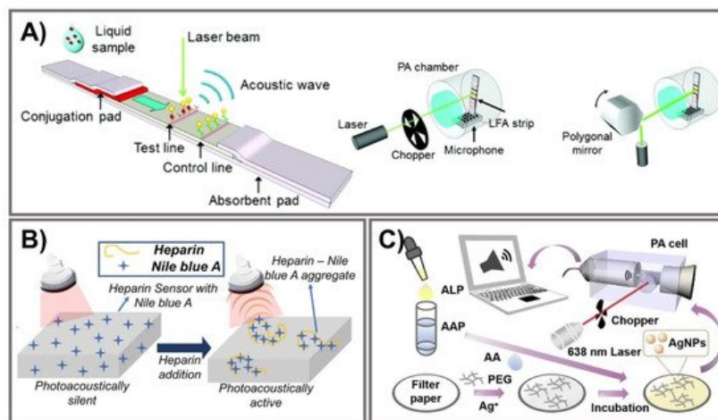
Figure 5. Photoacoustic signal amplification. (A) From left to right, PA-based LFA strip illuminated by a laser beam to generate PA signals; illustration of PA measurement systems for chop mode and scan mode. Adapted with permission from Ref. [112]. (B) Illustration of a heparin sensor via interactions with Nile blue A to activate photoacoustic signals. Adapted with permission from Ref. [113]. (C) PA device for ALP detection via PA signal generation of AgNPs from hydrolyzed AAP on filter paper. Adapted with permission from Ref. [114].
