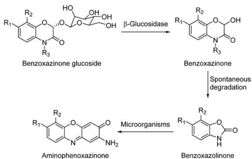
Scheme 1. General degradation process of benzoxazinones.
