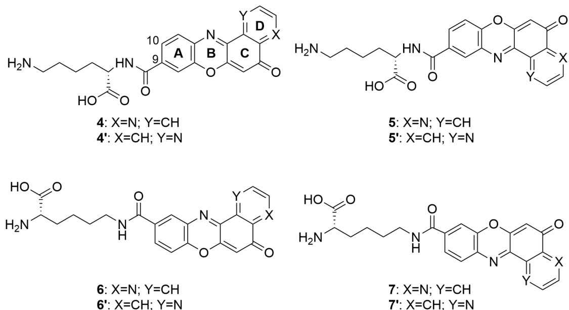
Figure 6. Structure of the pyridophenoxazinone derivatives conjugated to L-lysine.
