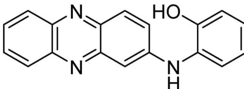
Figure 4. Structure of N -(2-hydroxyphenyl)-2-phenazinamine (NHP).
