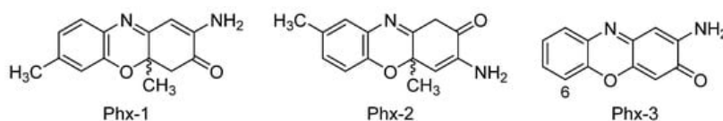
Figure 3. Most studied aminophenoxazinones: 2-amino-4,4a-dihydro-4a,7-dimethyl-3H-phenoxazin-3-one (Phx-1), 3-amino-1,4a-dihydro-4a,8-dimethyl-2H-phenoxazin-2-one (Phx-2) and 2-aminophenoxazine-3-one (Phx-3).
