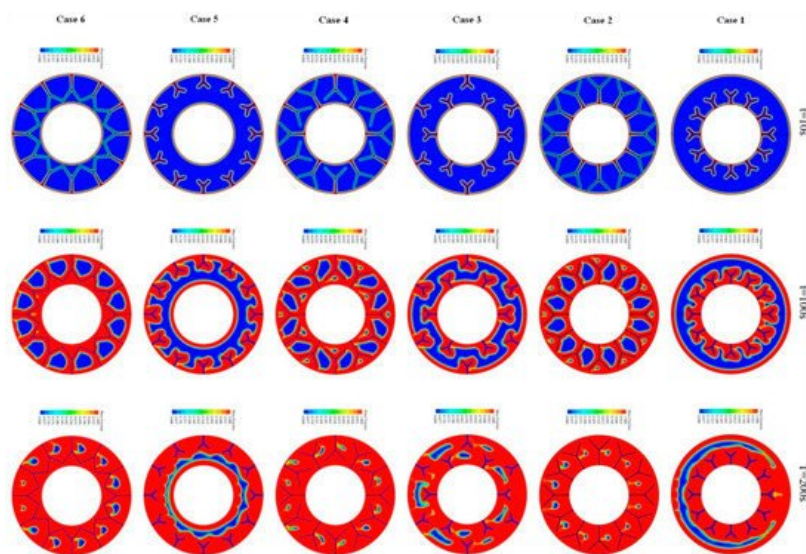
Figure 8. The liquid fraction in the six different cases at different times. (Copyright 2020 Elsevier) [42].
