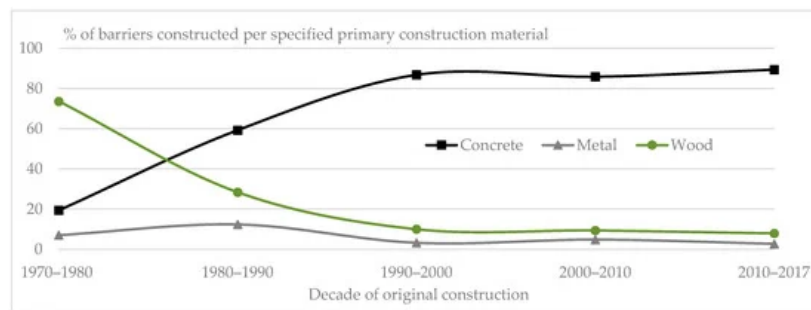
Figure 1. Panel material trends during the last five decades of road traffic noise wall construction (from 1973 to 2017).
