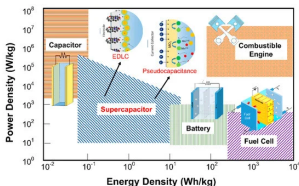
Figure 1. Ragone plot for several types of electrochemical energy storage devices: adapted from Reference [5]. Copyright American Chemical Society, 2004.
