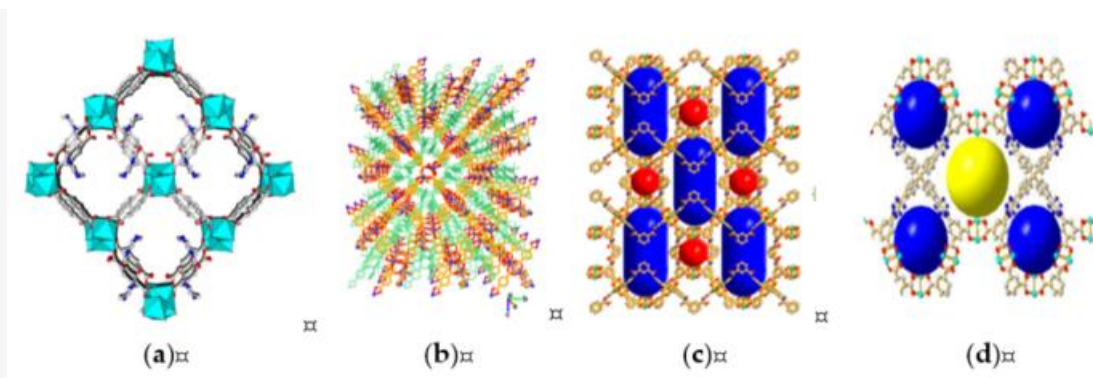
Figure 8. The 3D structure of MOFs: (a) \text{In}_2(\text{OH})(\text{btc})(\text{Hbtc})_{0.4}(\text{L})_{0.6}\cdot 3\text{H}_2\text{O} (reprinted with permission from Liu, L.; Wang, S.M.; Han, Z.B.; Ding, M.; Yuan, D.Q.; Jiang, H.L. Exceptionally Robust In-Based Metal-Organic Framework for Highly Efficient Carbon Dioxide Capture and Conversion. Inorg. Chem. 2016 , 55 , 3558–3565. Copyright (2016) American Chemical Society.); (b) [\{\text{Co}(\text{BDC})(\text{L})\cdot 2\text{H}_2\text{O}\cdot x\text{G}\}]_n (CoMOF-2) (reprinted with permission from Parmar, B.; Patel, P.; Pillai, R.S.; Tak, R.K.; Kureshy, R.I.; Khan, N.H.; Suresh, E. Cycloaddition of \text{CO}_2 with an Epoxide-Bearing Oxindole Scaffold by a Metal–Organic Framework-Based Heterogeneous Catalyst under Ambient Conditions. Inorg. Chem. 2019 , 58 , 10084–10096. Copyright (2019) American Chemical Society.); (c) \{\text{Cu}_2[(\text{C}_{20}\text{H}_{12}\text{N}_2\text{O}_2)(\text{COO})_4]\}_n (reprinted with permission from Li, P.Z.; Wang, X.J.; Liu, J.; Phang, H.S.; Li, Y.; Zhao, Y. Highly Effective Carbon Fixation via Catalytic Conversion of \text{CO}_2 by an Acylamide-Containing Metal-Organic Framework. Chem. Mater. 2017 , 29 , 9256–9261. Copyright (2017) American Chemical Society.); (d) \{\text{Cu}_4[(\text{C}_{57}\text{H}_{32}\text{N}_{12})(\text{COO})_8]\}_n (reprinted with permission from Li, P.Z.; Wang, X.J.; Liu, J.; Lim, J.S.; Zou, R.; Zhao, Y. A Triazole-Containing Metal-Organic Framework as a Highly Effective and Substrate Size-Dependent Catalyst for \text{CO}_2 Conversion. J. Am. Chem. Soc. 2016 , 138 , 2142–2145. Copyright (2016) American Chemical Society.).
