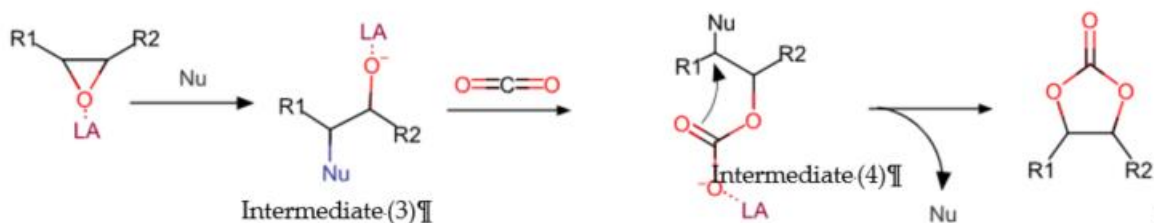
Figure 4. Reaction mechanistic pathways of cycloaddition of epoxide with \text{CO}_2 .
