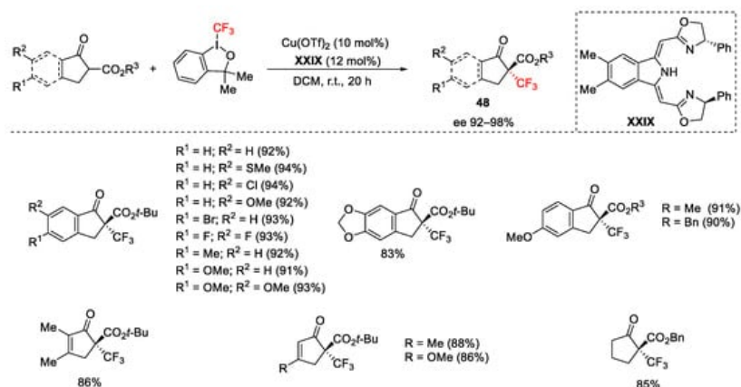
Scheme 51. Trifluoromethylation of β-ketoesters.
