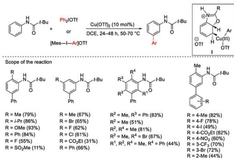
Scheme 1. \text{Cu}(\text{OTf})_2 -catalyzed arylation of pivanilides.
