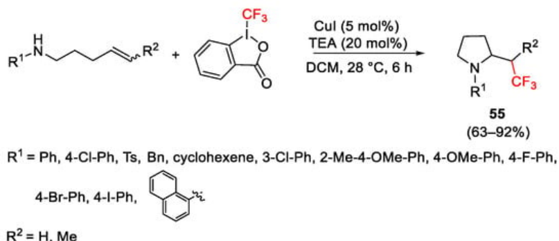
Scheme 67. Synthesis of β-trifluoromethylamines.
