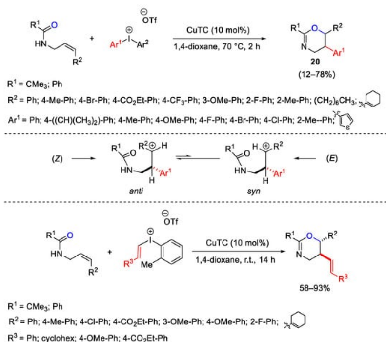
Scheme 26. Oxyarylation and oxyvinylation of allyl amides with diaryl- and vinyl(aryl)iodonium triflates.
