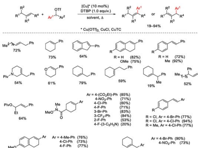
Scheme 16. Copper-catalyzed arylation of alkenes with diaryliodonium salts.
