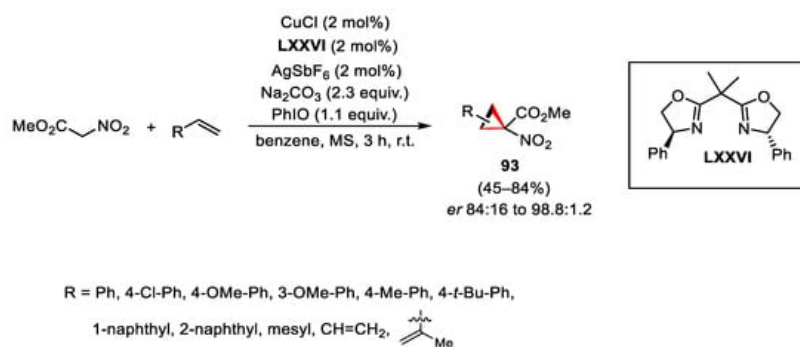
Scheme 131. Copper-catalyzed cyclopropanation reaction.
