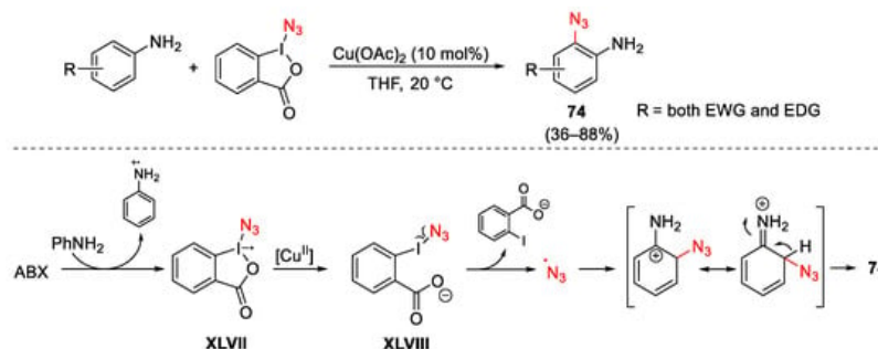
Scheme 99. Direct C–H azidation of anilines with ABX under copper catalysis.
