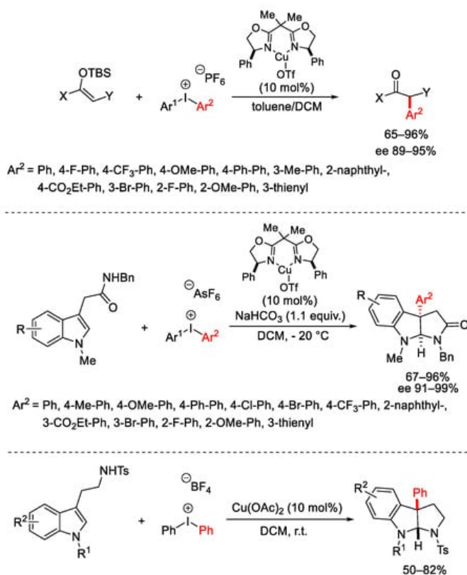
Scheme 14. \alpha -Arylation of enolsilanes and indole 3-acetamides.
