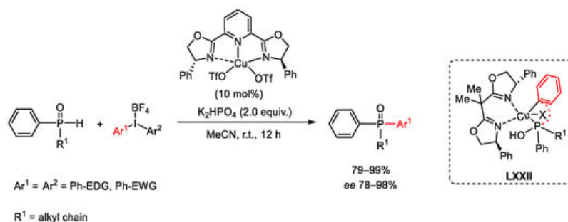
Scheme 126. Enantioselective copper-catalyzed P-Arylation using diaryliodonium reagents.
