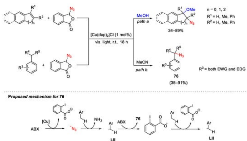
Scheme 102. Azidation of styrene-type double bond ( path a ) and benzylic C-H bonds ( path b ) with ABX under copper-photoredox catalysis.
