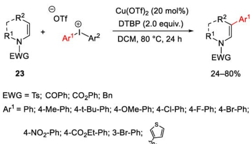
Scheme 28. \text{Cu}(\text{OTf})_2 -catalyzed \beta -arylation of enamides.
