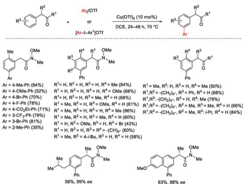
Scheme 2. \text{Cu}(\text{OTf})_2 -catalyzed arylation of \alpha -aryl-substituted carbonyl compounds.
