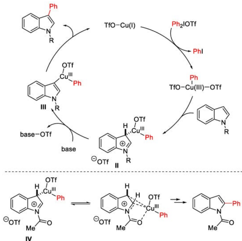
Scheme 6. Proposed mechanism for the selective \text{Cu}(\text{OTf})_2 -catalyzed C3 arylation of indoles vs. C2-arylation of N -acetylindoles.
