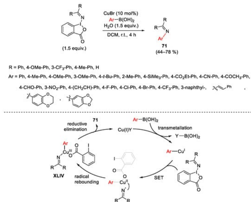
Scheme 96. Copper-catalyzed synthesis of N -aryl(alkenyl) imines using hypervalent iodane (III) reagent containing (diarylmethylene)amino groups.
