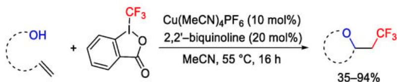
Scheme 69. Oxytrifluoromethylation of unactivated alkenes.
