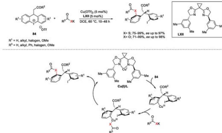
Scheme 115. Cu-catalyzed enantioselective diarylmethanes formation.
