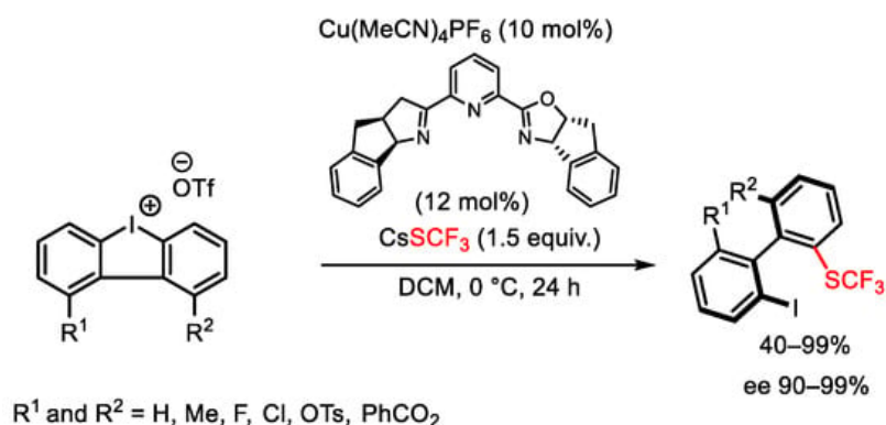
Scheme 120. Atroposelective synthesis of trifluoromethylthiolated biaryls.
