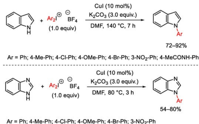
Scheme 78. Copper(I)-catalyzed arylation of indole and benzimidazole.
