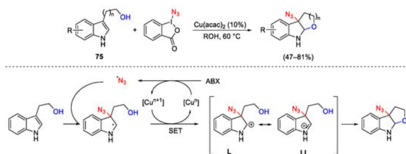
Scheme 101. Intramolecular copper-catalyzed alkoxyazidation of tryptophols.
