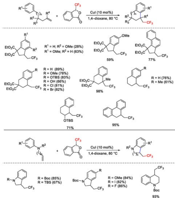
Scheme 75. Domino C-C and C- \text{CF}_3 bond formations.
