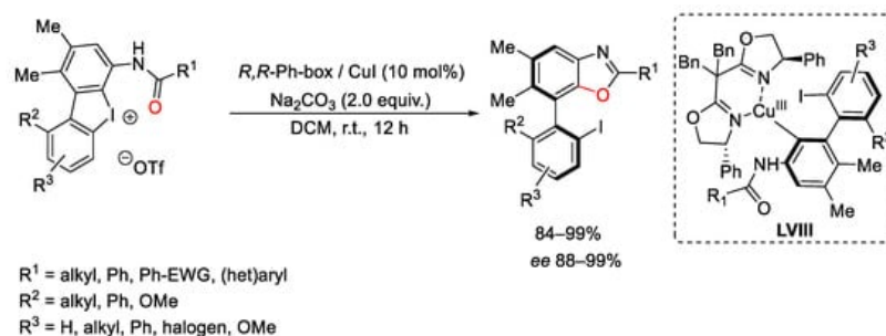
Scheme 111. Copper-catalyzed benzoxazoles formation with cyclic diaryliodonium compounds.
