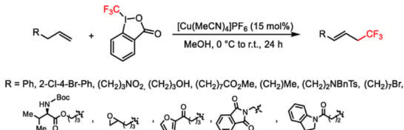
Scheme 41. Trifluoromethylation of terminal alkenes.
