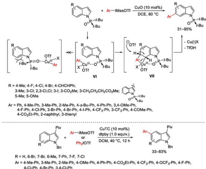
Scheme 8. Selective C5- and C6-arylation of substituted indoles.
