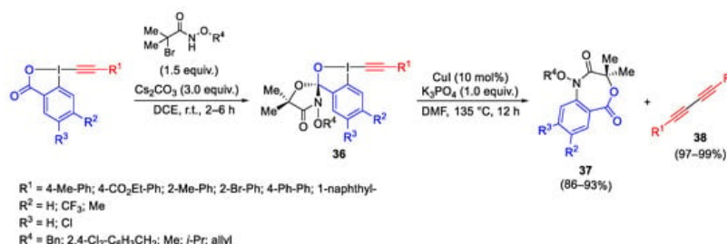
Scheme 39. Synthesis and reactivity of cyclic \lambda^3 -iodanes.
