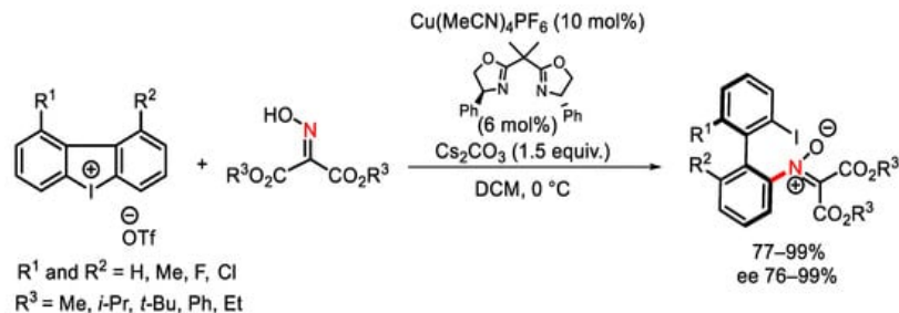
Scheme 95. Copper-catalyzed synthesis of atropisomeric nitrones.
