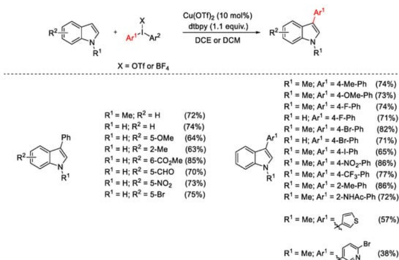
Scheme 4. Cu(OTf) 2 -catalyzed C3-arylation of indoles.
