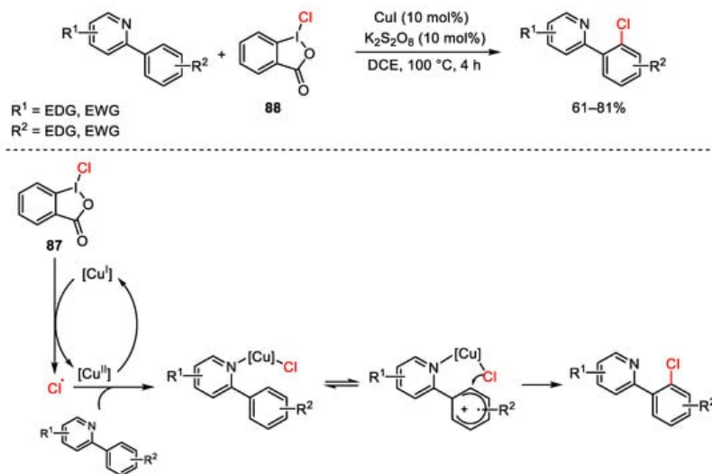
Scheme 123. Regioselective chlorination of C-H aromatic bonds.
