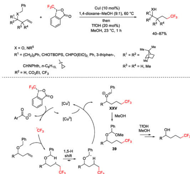
Scheme 42. Trifluoromethylation of homoallylic alcohol derivatives.
