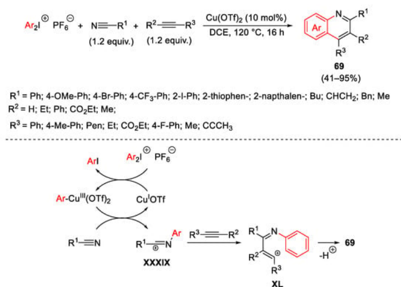
Scheme 92. Copper-catalyzed synthesis of substituted quinolones 69 by a three-component cascade annulation.
