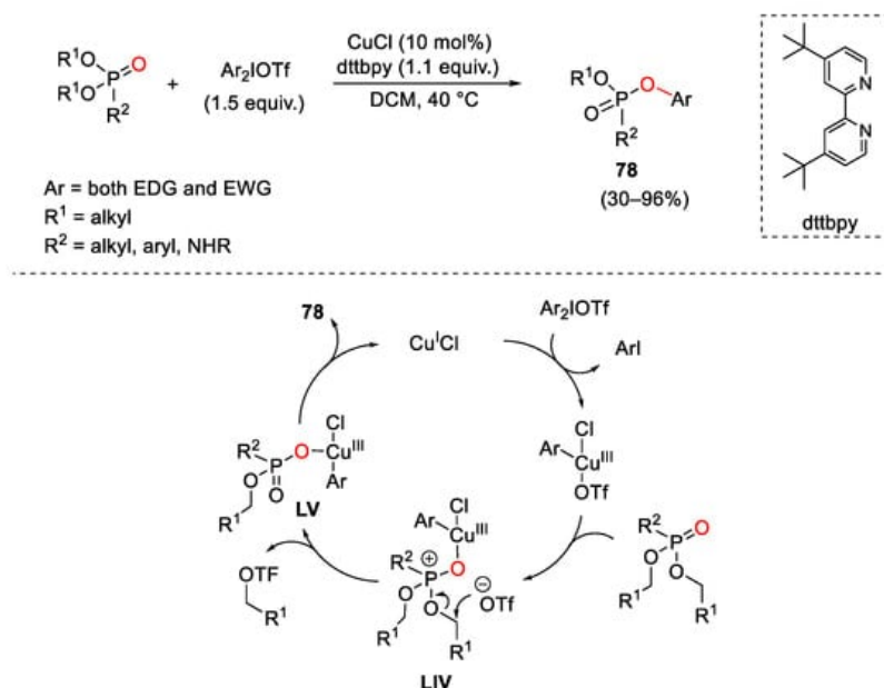
Scheme 107. Copper(I)-catalyzed C-H oxyarylation of phosphonates with diaryliodonium triflates reagents.
