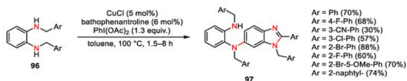
Scheme 135. Dimerization/cyclization of N,N' -dibenzyl-1,2-benzenediamines.
