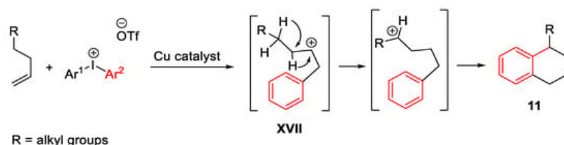
Scheme 21. Copper-catalyzed arylation of alkenes with diaryliodonium salts.
