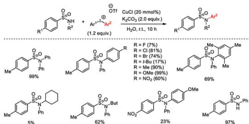
Scheme 82. Copper(I)-catalyzed arylation of sulfonamides with diaryliodonium salts.
