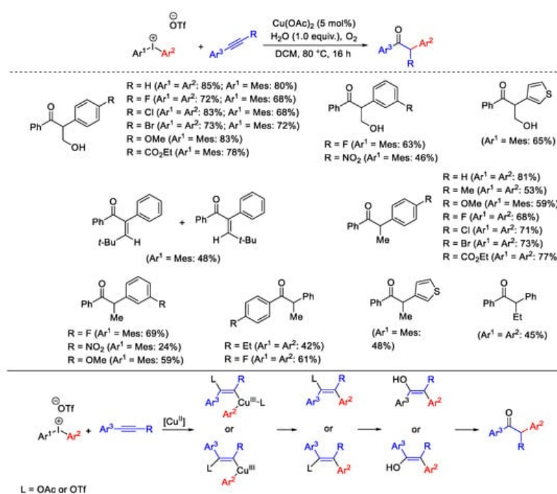
Scheme 19. Arylation reaction of internal alkynes with diaryliodonium salts to \alpha -arylketoones.
