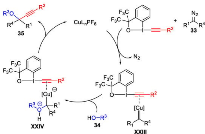
Scheme 36. Proposed mechanism for the three-component oxyalkynylation reaction.
