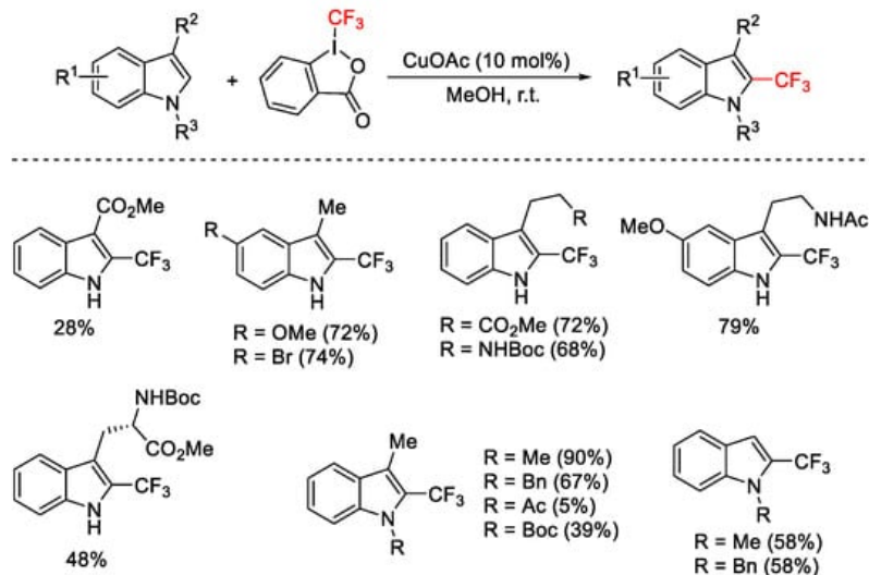
Scheme 62. Trifluoromethylation of C2 position of indoles.
