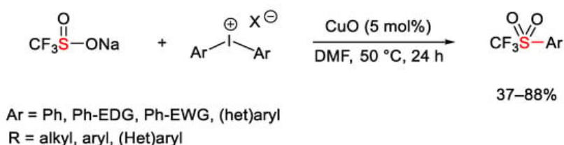
Scheme 116. Copper-catalyzed synthesis of aryltrifluoromethylsulfones.
