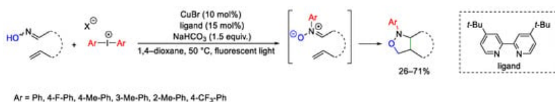
Scheme 97. Copper-catalyzed synthesis of N -aryl-isoxazolidines.
