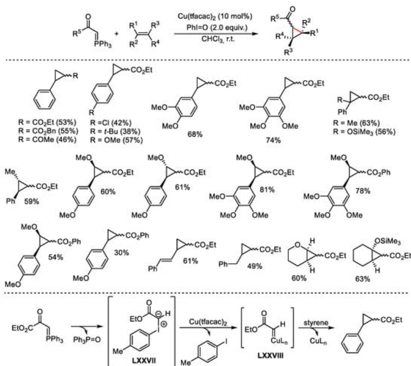
Scheme 132. Cyclopropanation of alkenes in the presence of catalytic Cu(tfacac) 2 and iodosotoluene.
