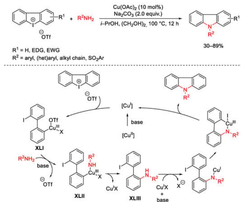
Scheme 94. One-pot copper-catalyzed amine insertion into cyclic diaryliodonium reagents.
