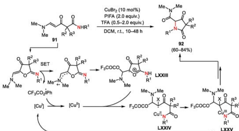
Scheme 130. Plausible mechanism for the formation of pyrrolidine-2,4-diones.
