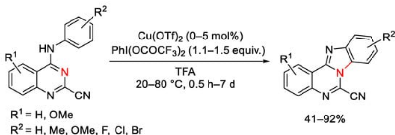
Scheme 128. Copper(II)-mediated oxidative ring closure of 4-anilinoquinazoline-2-carbonitriles.
