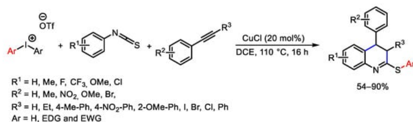
Scheme 121. Synthesis of quinoline derivatives.
