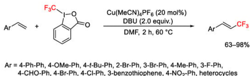
Scheme 45. Trifluoromethylation of styrenes.
