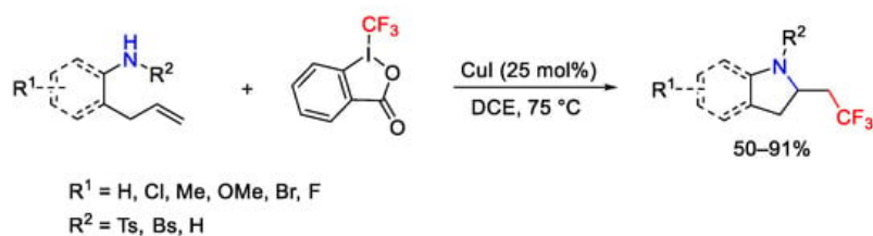
Scheme 76. Aminotrifluoromethylation of unactivated alkenes.
