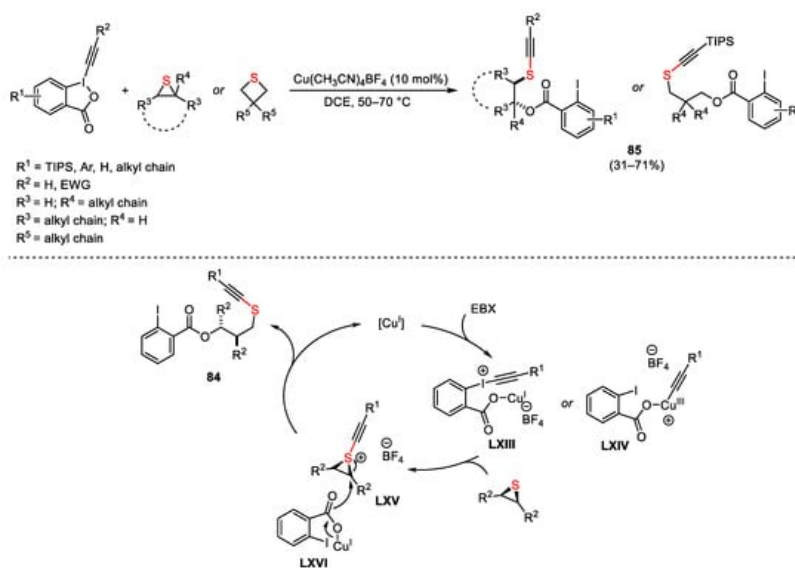
Scheme 117. Copper-catalyzed ring opening of sulphur heterocycles using EBX reagent.
