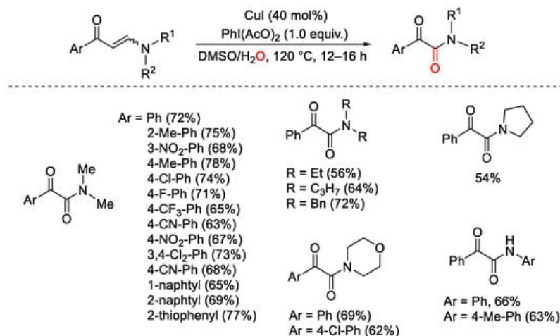
Scheme 133. Synthesis of \alpha -keto amides from enaminones under the copper/PhI(OAc) 2 catalytic system.
