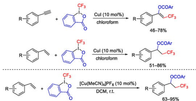
Scheme 63. Oxytrifluoromethylation of alkenes and alkynes.
