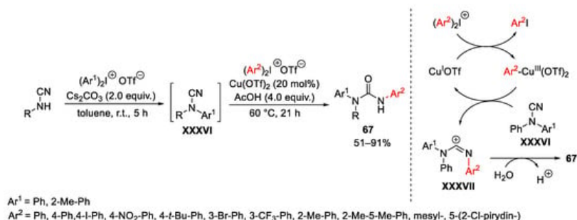
Scheme 89. Copper-catalyzed synthesis of unsymmetrical diarylureas.
