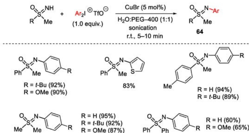
Scheme 83. Copper(I)-catalyzed arylation of sulfoximines with diaryliodonium salts.
