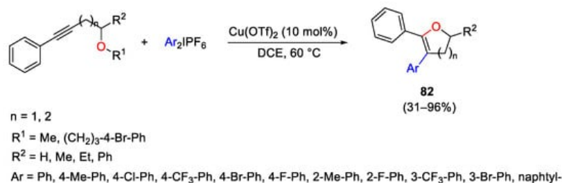
Scheme 113. Copper-catalyzed intramolecular aryl-etherification of alkoxy alkynes.
