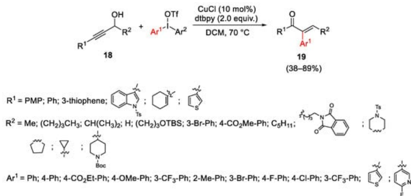
Scheme 25. Copper-catalyzed Meyer–Schuster rearrangement of propargyl alcohols.
