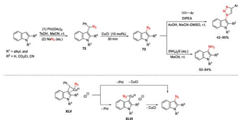
Scheme 98. Copper-catalyzed azidation of indoles.
