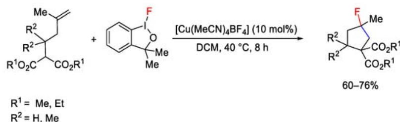
Scheme 122. Hypervalent iodine as reagent in fluorocyclization.
