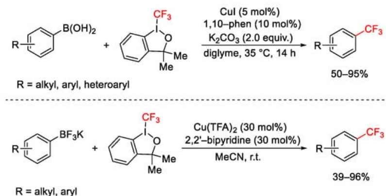
Scheme 60. Trifluoromethylation of organo boronic acids and organotrifluoroborates.
