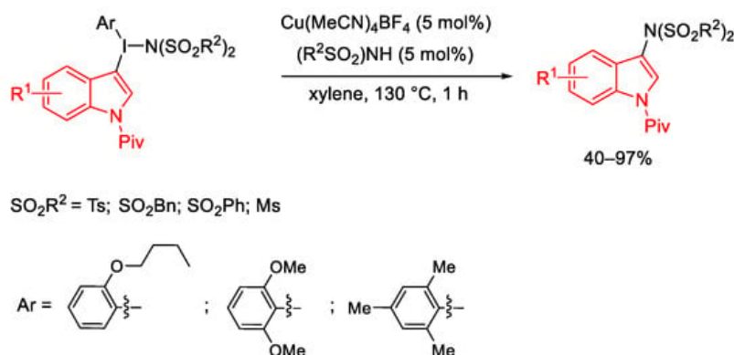
Scheme 84. Copper(I)-catalyzed C-N coupling reaction using indolyl(aryl)iodonium imides.
