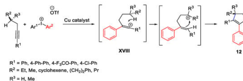
Scheme 22. Copper-catalyzed arylation of alkynes with diaryliodonium salts.
