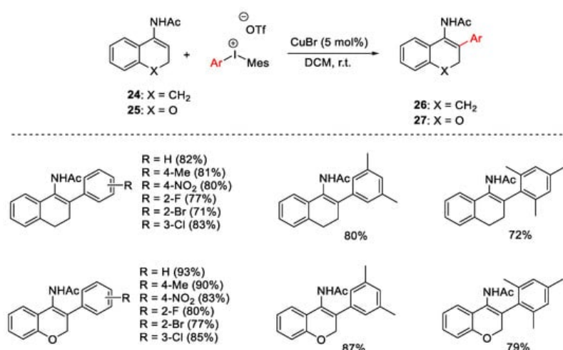
Scheme 29. \beta -Arylation of secondary cyclic enamides.
