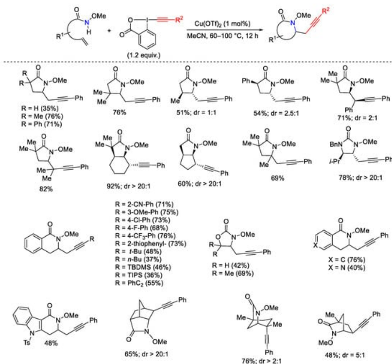
Scheme 37. Cu-catalyzed aminoalkynylation of alkenes with EBX.
