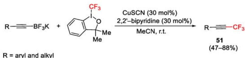
Scheme 61. Trifluoromethylation of alkynyltrifluoroborates.
