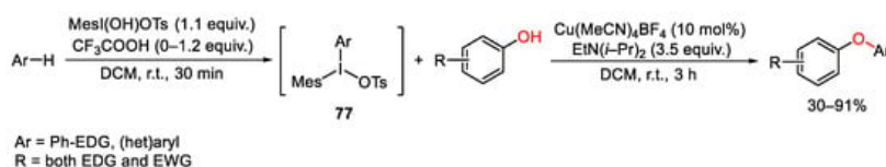
Scheme 104. Copper(I)-catalyzed C-H oxyarylation of phenol derivatives.
