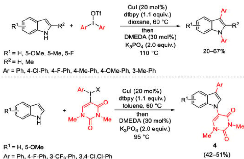
Scheme 9. Tandem diarylation of indoles.
