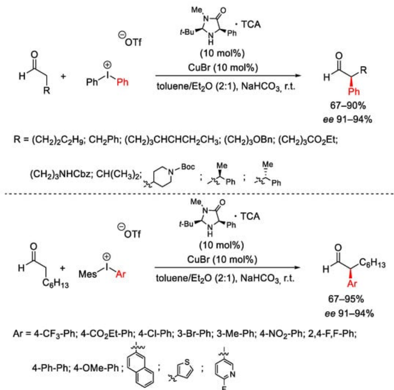
Scheme 10. Stereoselective arylation of enolizable aldehydes.
