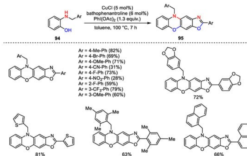
Scheme 134. Dimerization/cyclization of 2-benzylaminophenols.
