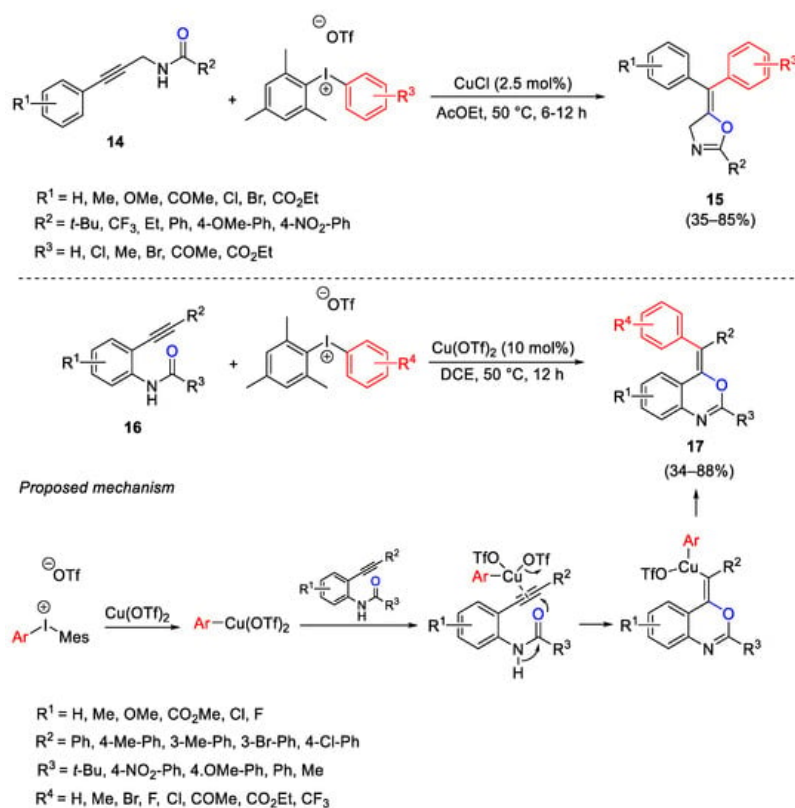
Scheme 24. Carboarylation of propargylamides and 2-ethynylanilides for the construction of oxazolines and benzoxazines.
