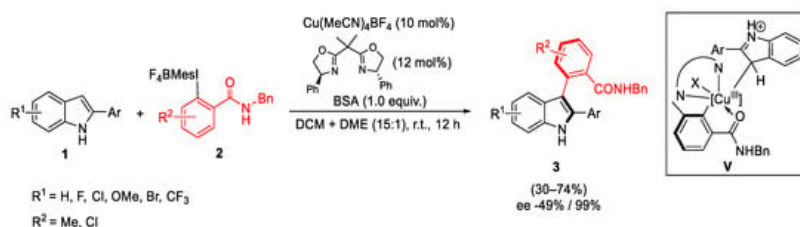
Scheme 7. Atroposelective synthesis of 2,3-diarylindoles.
