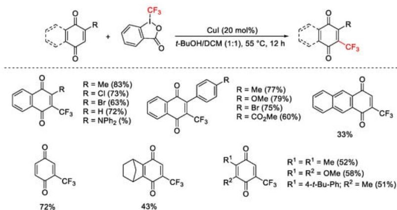
Scheme 50. Trifluoromethylation of quinones.
