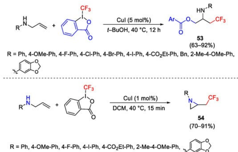
Scheme 66. Synthesis of β-trifluoromethylamines.
