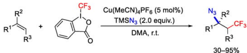
Scheme 65. Copper mediated trifluoromethylazidation of alkenes.
