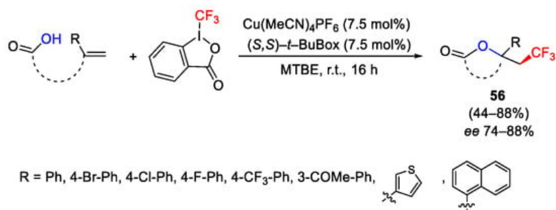
Scheme 70. Asymmetric oxytrifluoromethylation of alkenes.
