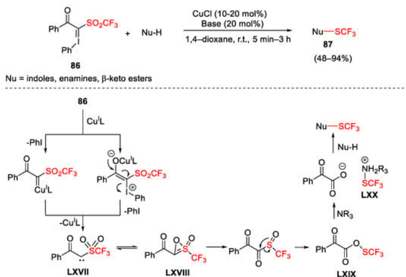
Scheme 119. Copper-catalyzed trifluoromethyl thiolation of nucleophiles with hypervalent iodonium ylide.
