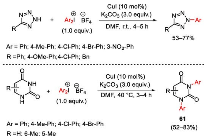
Scheme 79. Copper(I)-catalyzed arylation of tetrazole and uracil derivatives.
