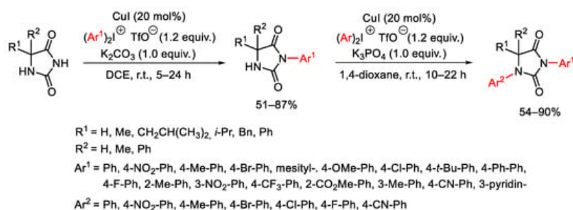
Scheme 81. Copper(I)-catalyzed arylation of hydantoins.
