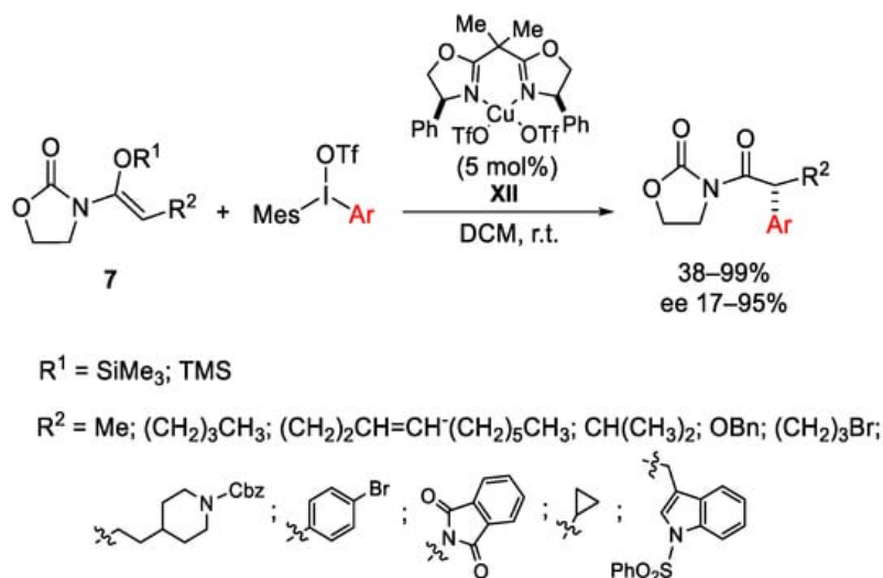
Scheme 13. Enantioselective \alpha -arylation of N -acyloxazolidinones.
