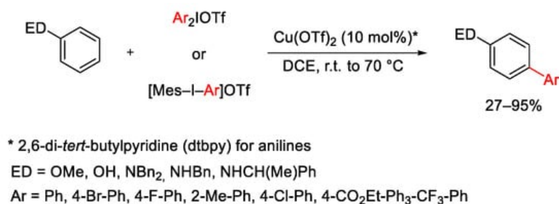
Scheme 3. Cu(OTf) 2 -catalyzed arylation of electron-rich arenes.
