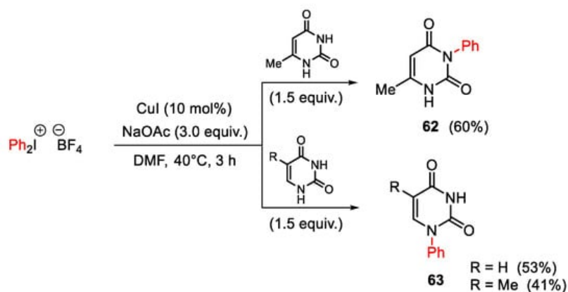
Scheme 80. Regioselective copper(I)-catalyzed arylation of 6-methyluracile, thymine and uracil.
