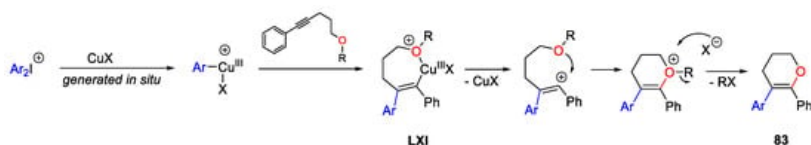
Scheme 114. Possible mechanism for the intramolecular aryl-etherification of alkoxy alkynes.
