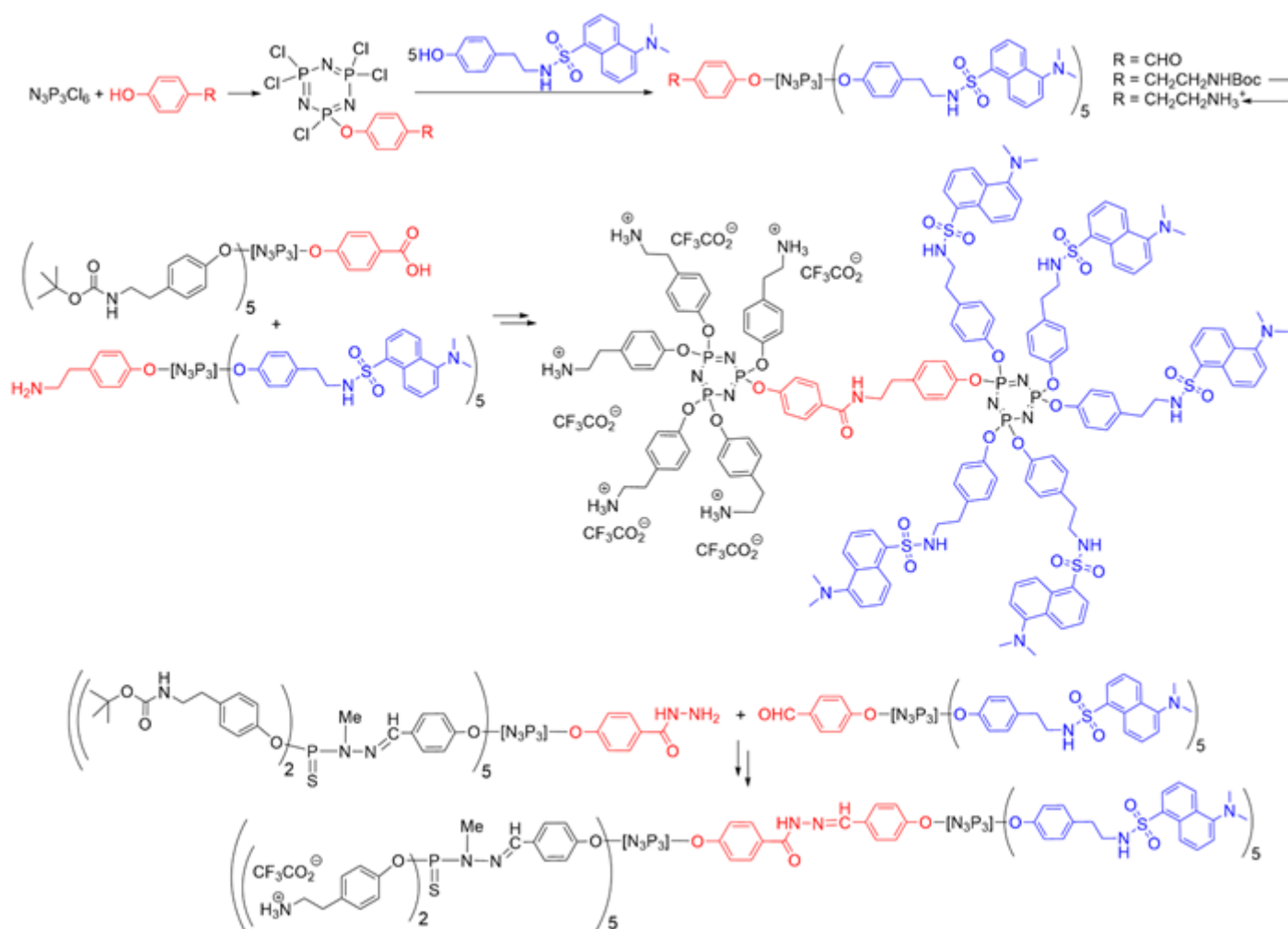
Scheme 3. Synthesis of fluorescent dendrons, and their association with other dendrons based on N_3P_3 for the synthesis of two types of Janus dendrimers.
