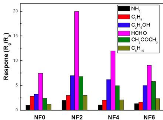
Figure 5. Responses of the sensors to 100 ppm different gases at their optimum working temperature; LaFeO 3 nanofibers doped by different amounts of Ag were marked as NF0 , NF2 , NF4 and NF6 (reproduced with the permission from reference [104]).
