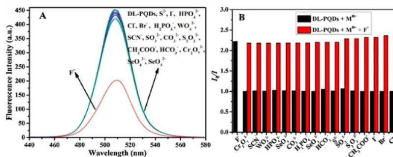
Figure 15. (A) Fluorescence response of dual ligand capped perovskite quantum dots (DL-PQDs) to different anions and \text{F}^- (90 \mu\text{M} for \text{F}^- and 450 \mu\text{M} for other anions). (B) Interference studies of the novel nanosensor toward \text{F}^- . The black bars represent the fluorescence response of DL-PQDs to \text{F}^- and other anions (90 \mu\text{M} for \text{F}^- , 450 \mu\text{M} for other anions). The red bars represent the change of emission occurred after the subsequent addition of 90 \mu\text{M} of \text{F}^- to the above solutions (reproduced with the permission from reference [151]).
