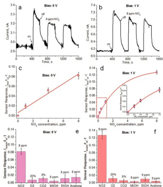
Figure 17. Room-temperature chemical response of the FMCPiB devices in the self- and externally-powered mode. Dynamic sensor response of an FMCPiB device to three consecutive injection of 8 ppm NO 2 (a) self-powered under weak fluorescent lamp light irradiation (1.3 \mu\text{W cm}^{-2} ) and (b) externally powered with 1 V bias in the dark. FMCPiB sensor response as a function of the NO 2 concentration; (c) in the self-powered mode and (d) at the 1 V external bias; the inset in (d) is the enlarged part of the red dashed region. The sensor response of the FMCPiB sensor for six different gases (e) in the self-powered operational mode; and (f) at the 1 V external bias. The gas sensing measurements were conducted at room temperature (30 °C) under simulated air ( V_{\text{N}_2}/V_{\text{O}_2} = 4 ) with a constant total gas flow of 0.5 L min -1 (reproduced with the permission from reference [166]).
