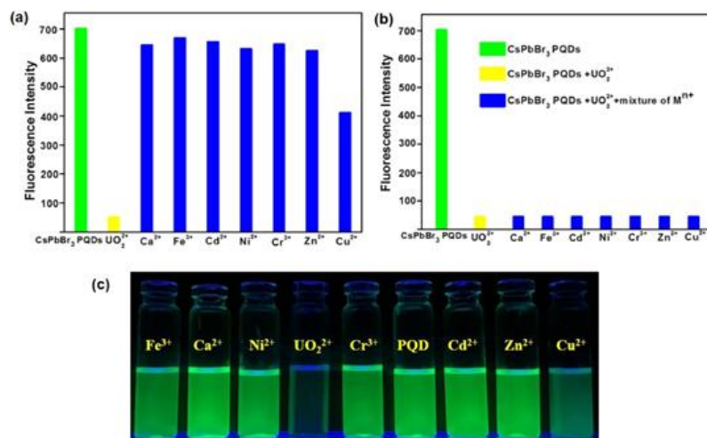
Figure 9. (a) Change in the PL of CsPbBr 3 PQDs upon the addition of various ions. (b) Effect of interfering cations with the absorption of bare CsPbBr 3 PQDs and CsPbBr 3 PQDs + UO 2 2+ complex (c) Digital photograph of colorimetric changes of the probe upon addition of various metal ions (reproduced with the permission from reference [133]).
