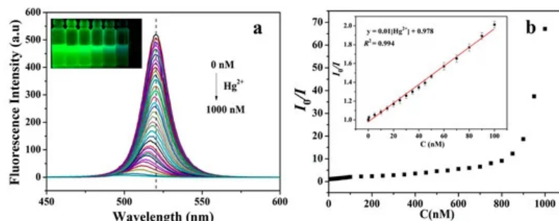
Figure 14. (a) Evolution of fluorescence spectra changes of \text{CH}_3\text{NH}_3\text{PbBr}_3 QDs upon the addition of different amounts of \text{Hg}^{2+} . The concentration of \text{Hg}^{2+} from top to bottom: 0–1000 nM. (b) Linear fitting curve of I_0/I with respect to \text{Hg}^{2+} concentration over the range of 0–100 nM (reproduced with the permission from reference [148]).
