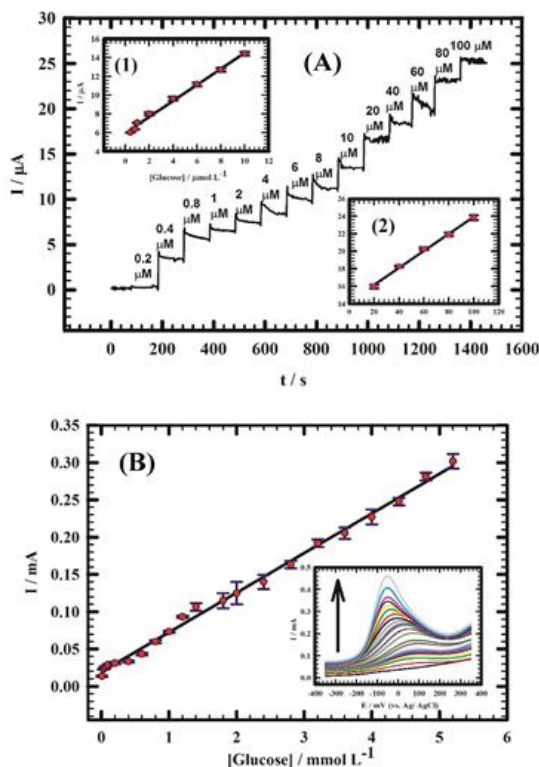
Figure 6. (A) Amperometric response of graphite/ \text{Sr}_2\text{Pd}_{0.7}\text{Au}_{0.3}\text{O}_3 with successive additions of glucose from 0.2 to 100 \mu\text{M} . Insets (1, 2): calibration curves for glucose for concentrations from 0.4 to 10 \mu\text{M} and from 20 to 100 \mu\text{M} , respectively.
