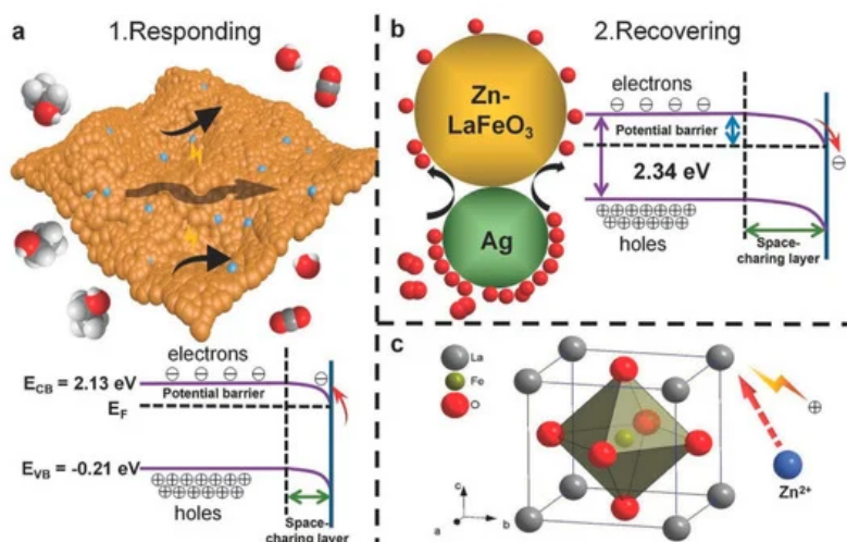
Figure 18. Schematic illustration of the sensing mechanism of the AZLFO-based sensors to ethanol: (a) exposed to ethanol; (b) exposed to air and (c) Zn 2+ doping in the lattice of LFO (reproduced with the permission from reference [176]).
