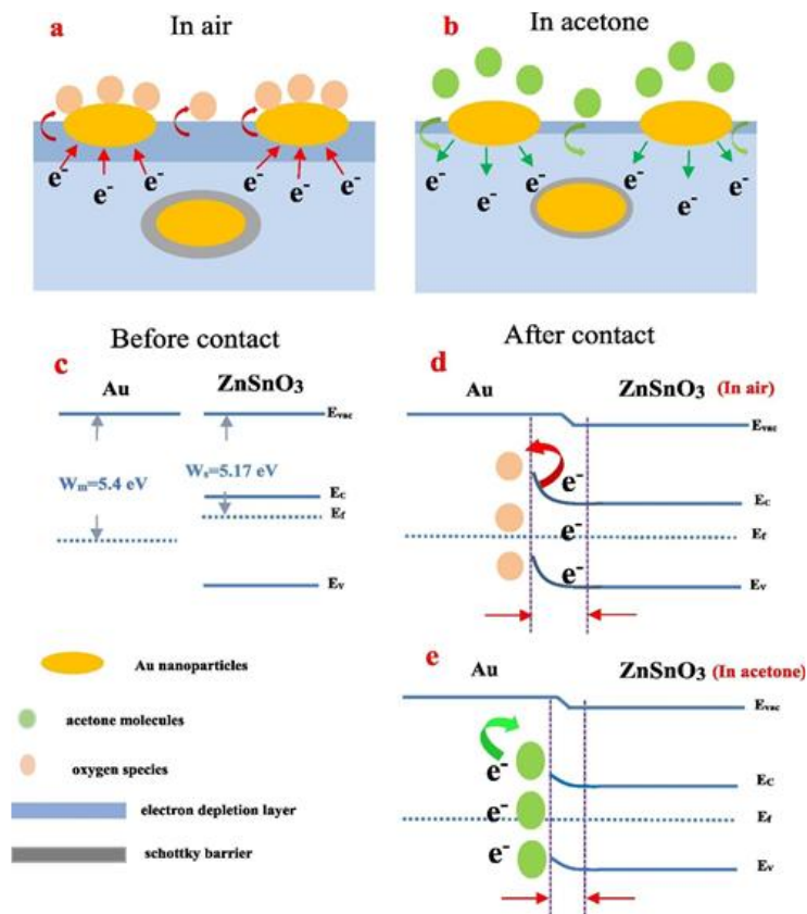
Figure 4. (a)-(e) Schematic illustration of the sensing mechanism of 0.25 Au/In-doped ZnSnO 3 sensor representing the Au enhanced electron generation in the presence of acetone (reproduced with the permission from reference [100]).
