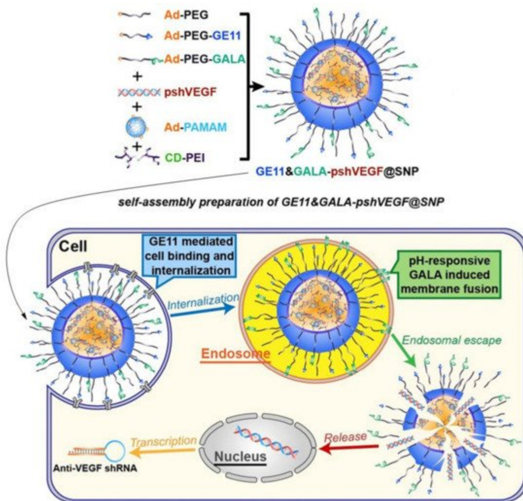
Figure 8. Schematic representation of the preparation and formation of self-assembly nanoparticle and transfection processes inside the cell. With the permission of [152].
