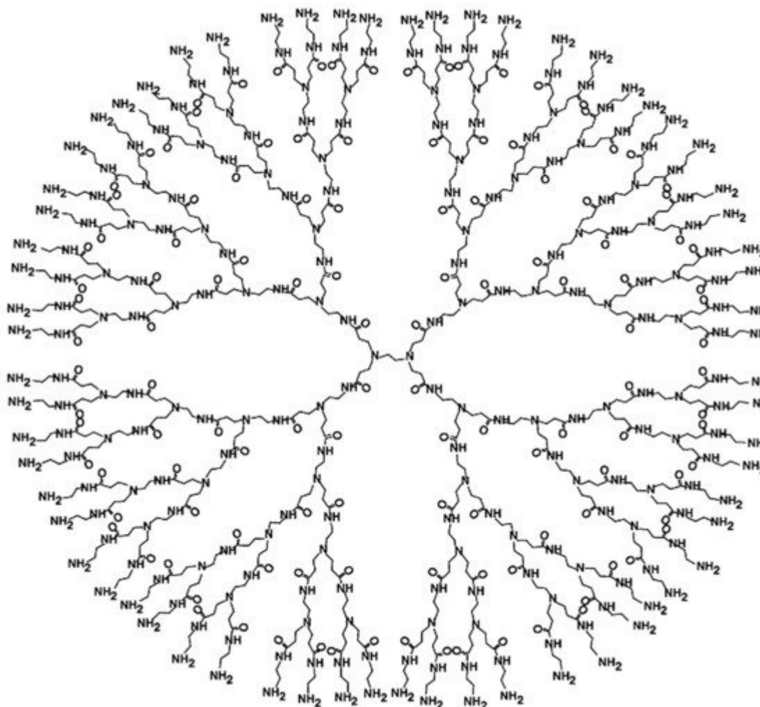
Figure 1. Chemical structure of poly(amidoamine) (PAMAM) G4. With the permission of [7] .
