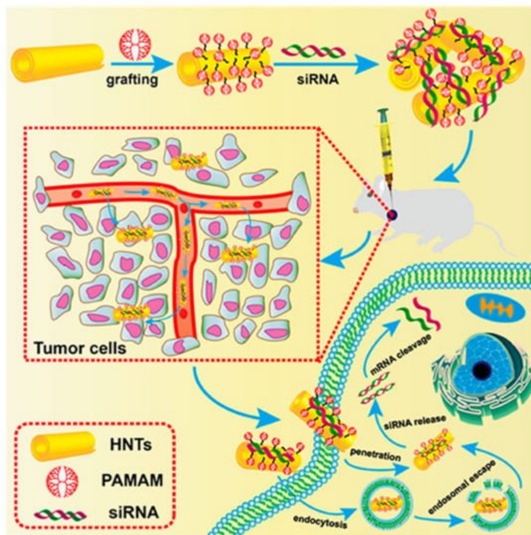
Figure 6. Schematic illustration for the preparation of PAMAM-g-HNTs/siRNA complex and its intracellular process in cancer cells. Reprinted with permission from [68], copyright (2021) American Chemical Society.
