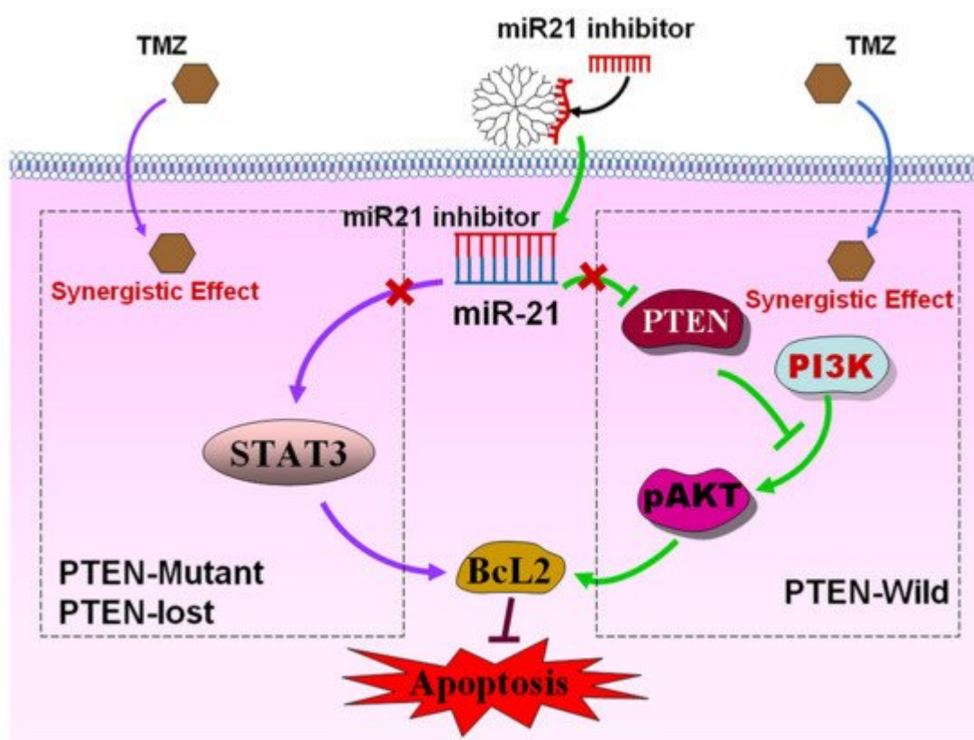
Figure 3. Mechanism of combination therapy for miR-21i and TMZ. miR-21i was delivered by PAMAM into the cells and coordinated with miR-21, leading to inactivation of miR-21. For LN229 cells (PTEN-wild), the inactivation of miR-21, which is inhibited by the simultaneous miR-21i and TMZ treatment, targets and reduces the expression of PTEN, blocks the PI3K-pAKT pathway, induces an increase in apoptosis, and leads to synergistic antiproliferative activity. For U251 (PTEN mutant) and U87 (PTEN-lost) cell lines with high STAT3 expression, the synergistic effect was achieved by sequence treatment of the two drugs. Reprinted with permission from [78] , copyright (2021) American Chemical Society.
