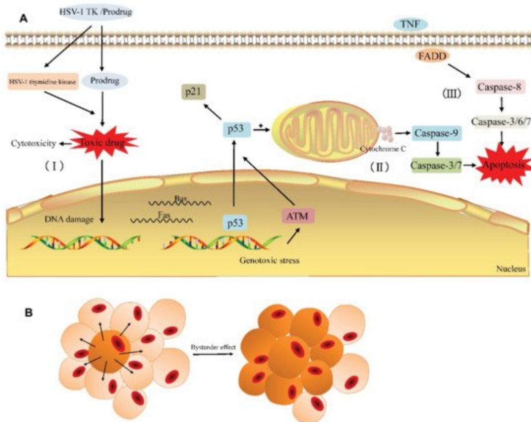
Figure 4. General principle of the HSV-TK suicide gene system. (A) The HSV-TK/prodrug-system-induced cytotoxicity and apoptosis in tumor cell. (I) The HSV-1 TK gene coding for thymidine kinase is delivered to the target cell. The expression of HSV-1 thymidine kinase and cellular kinases allows a prodrug (GCV) to be activated as the toxic drug (GCV-TP) in the cell and damage the DNA of the target cell. (II) Gene therapy induces endogenous apoptosis by activating p53 signaling pathway in the target cell. (III) Gene therapy induces exogenous apoptosis. (B) The bystander effect induces the death of adjacent cells. With the permission of [85].
