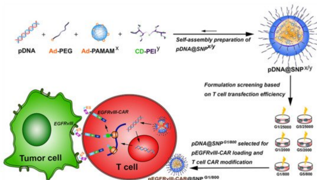
Figure 7. Schematic illustration of the preparation and formulation screening of pDNA@SNPs for pEGFRvIII-CAR loading and T cell CAR modification. Abbreviations: pDNA, plasmid DNA; Ad-PEG, adamantane-grafted poly(ethylene glycol); Ad-PAMAM x , adamantane-grafted polyamidoamine dendrimer (x: PAMAM dendrimer generation); CD-PEI y , cyclodextrin-grafted branched polyethylenimine (y: PEI molecular weight); SNPs, self-assembled nanoparticles; EGFRvIII, epidermal growth factor receptor variant III; CAR, chimeric antigen receptor;
