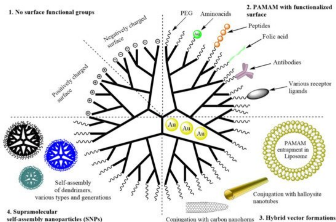
Figure 2. Schematic representation of the PAMAM dendrimer modification strategies covered in the review.
