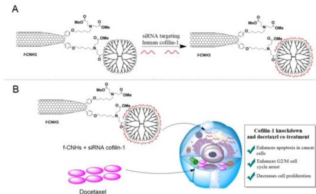
Figure 5. Schematic representation of an experiment involving the use of f-CNH3 hybrid nanovector. (A) Conjugation of f-CNH3 with siRNA targeted against human cofilin-1, a key protein in the regulation of cellular cytoskeleton. (B) Synergistic effects of siRNA against cofilin-1 and docetaxel on the LNCaP prostate cancer cell line. The f-CNH3-transported siRNA is released in the cell and inhibits cofilin-1 protein expression, leading to the "sensitization" of tumor cells to the effects of docetaxel treatment, resulting in widespread apoptosis, cell-cycle arrest at the G2/M phase, and subsequent inhibition of tumor cell proliferation. Adapted with the permission of [139].
