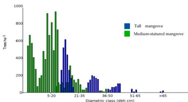
Figure 2. Number of trees (per ha -1 ) by diameter class (cm) in medium-statured and tall mangrove forests in the gulf of Guayaquil, Ecuador.
