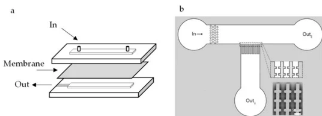
Figure 1. (a) Microfluidic configuration with an embedded membrane. (b) Microfluidic configuration with an array of parallel channels with the objective to mimic a membrane in an ideal situation. The image has been cropped and modified from the original work [32] and reproduced under the Creative Commons Attribution 4.0 International License [33].
