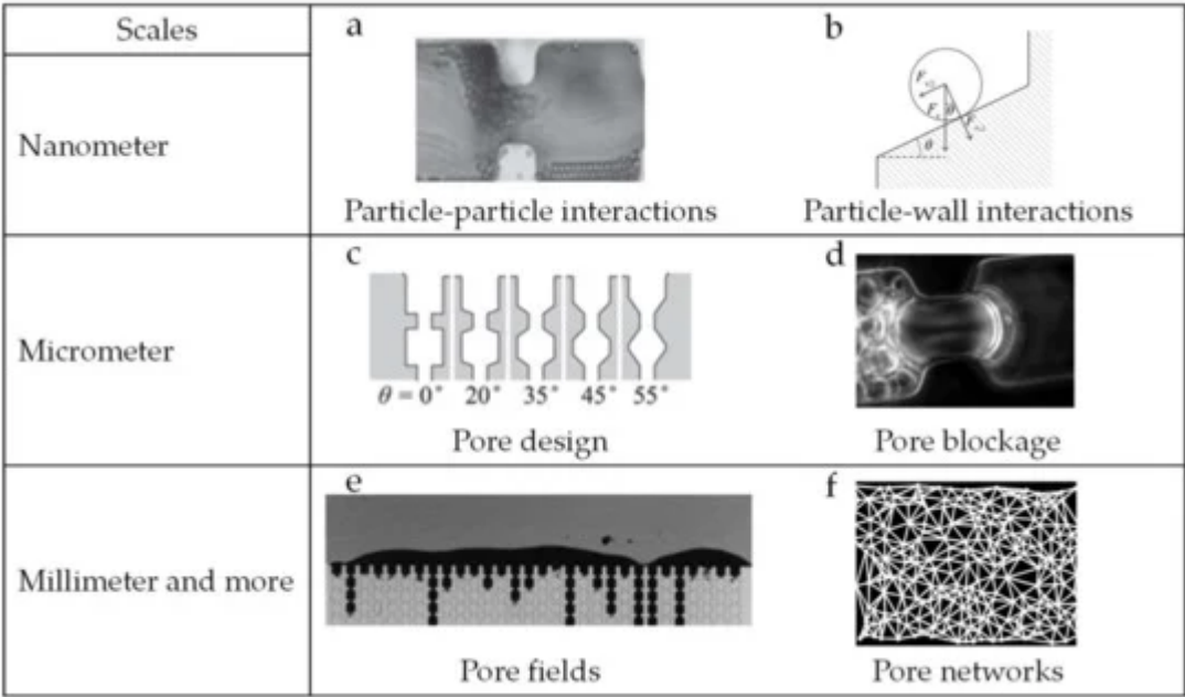
Figure 2. Examples of how microfluidic tools are applied to investigate mechanisms occurring at various scales. At nanometer scale particle–particle (a) and particle–wall (b) interactions can be studied [34]. Pore design (c) [34] and pore blockage (d) [35] are topics that can be investigated at micrometer scale, and finally at millimeter scale pore fields (e) [32] and pore networks (f) [36] have been used to study the collective behavior of particles in porous media. Images a-e have been cropped from their original work and reproduced under the Creative Commons Attribution 4.0 International License [33]. Image f has been reproduced with permission from the author.
