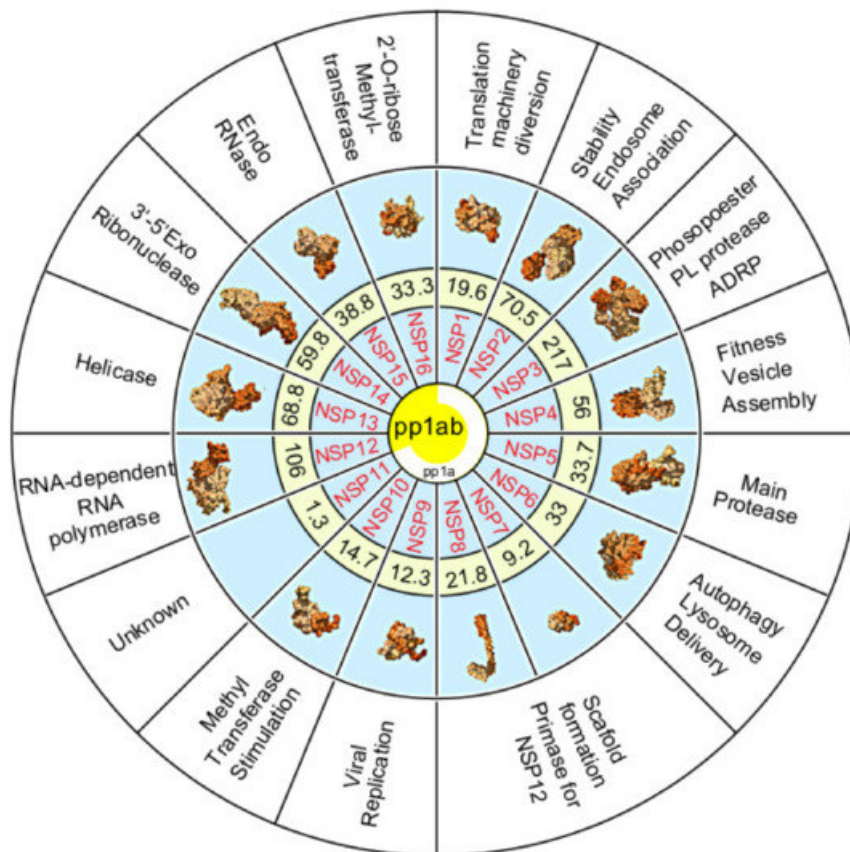
Figure 3. Summary diagram illustrating the non-structural proteins (Nsp) 1-16 cleaved from polyproteins pp1a (white partial circle) or pp1ab (yellow center). Numbers represent the molecular weight of Nsps in kilodaltons. Secondary structure prediction of each Nsp is shown except for Nsp11 which is unknown (Source PDB101.rcsb.org [30]). Nsp function is provided in the outer ring.
