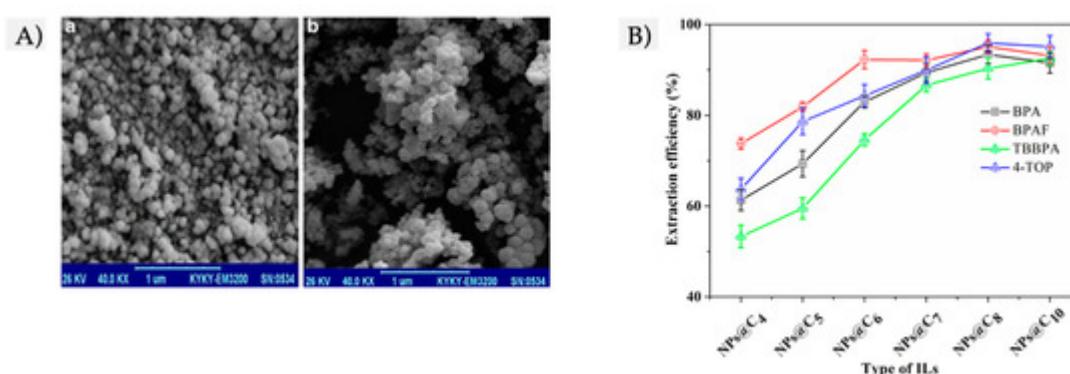
Figure 3. (A) SEM images of (a) \text{Fe}_3\text{O}_4 -based magnetic nanoparticles (MNPs), and (b) silica-coated \text{Fe}_3\text{O}_4 -based MNPs, used for the preparation of an ionic liquid (IL)-based FF. Figure adapted from [23] with permission of Springer. (B) Comparison between the extraction efficiencies obtained with different IL-based FFs with the same MNPs but different IL types (modifying the length of the alkyl chain of the IL cation), tested with a group of four endocrine-disrupting phenols. Figure adapted from [26] with permission of Elsevier.
