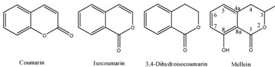
Figure 1. Structure of coumarin, isocoumarin, 3,4-dihydroisocoumarin and mellein.
