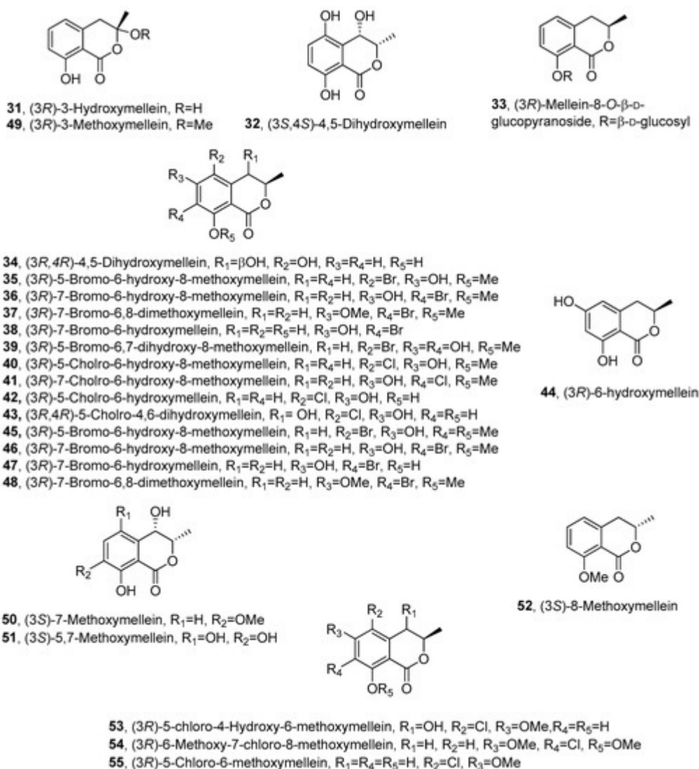
Figure 3. The structures of compounds 31 – 55 .
