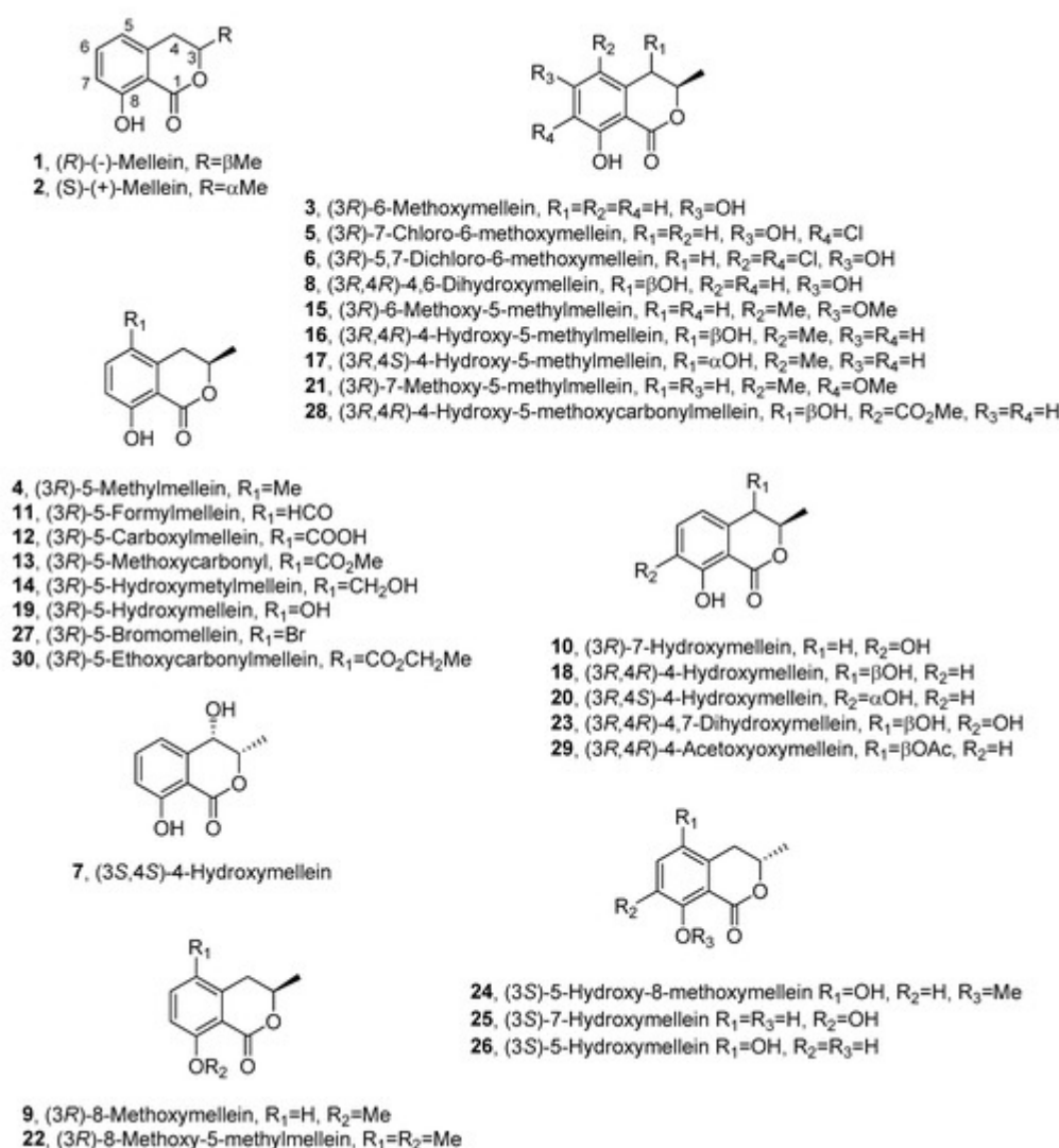
Figure 2. The structures of 1 – 30 .
