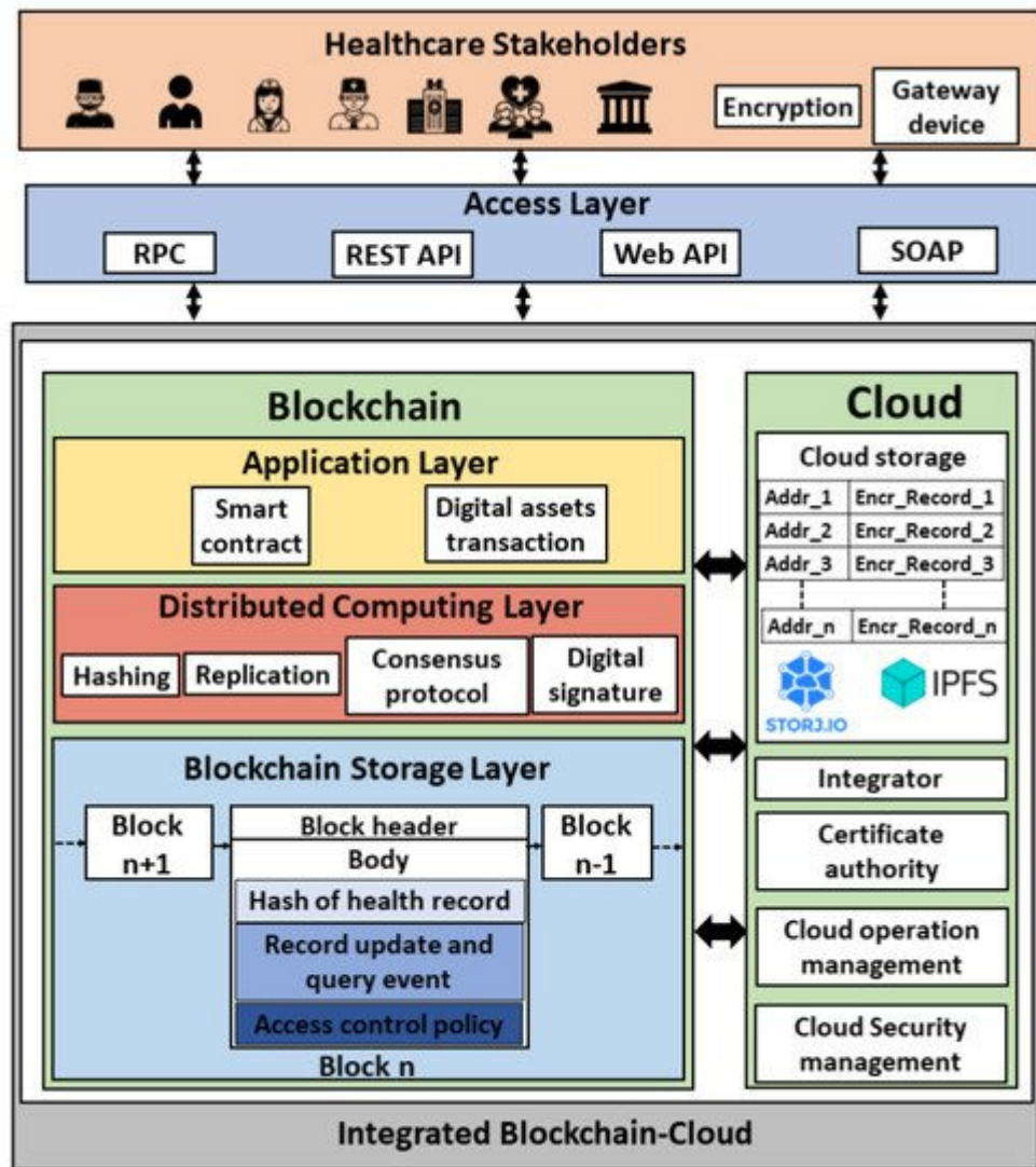
Figure 4. Non-encapsulated BcC architecture for healthcare.
