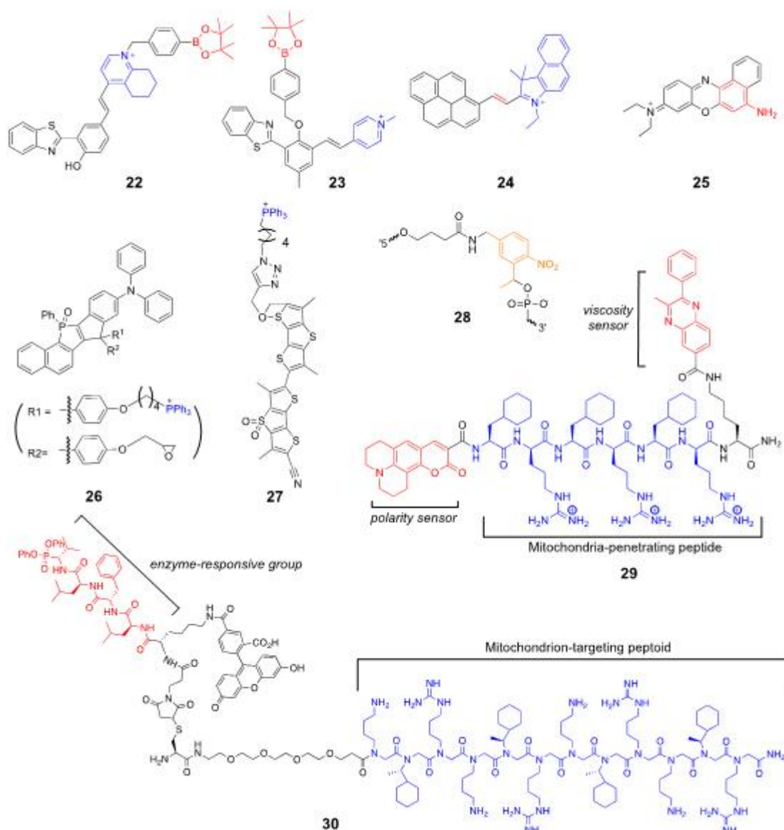
Figure 7. Mitochondrion-targeted probes.
