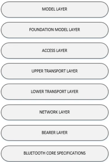
Figure 1. Bluetooth Low Energy (BLE) Mesh System Architecture [13].
