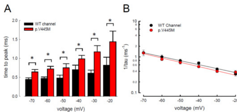
Figure 7. Slower time to peak of the resurgent Na + currents in the p.V445M mutant channel in the CHO-K1 cells (A) The time to the resurgent current peak was measured with the same protocol in Figure 4 ( n = 6 ). The time to the resurgent Na + current peak is significantly shortened in the WT than in the p.V445M mutant channel between -20 and -70 mV (*; p < 0.05 ). (B) The reciprocal of the time constants ( 1/\tau ) for the decay phase of resurgent Na + currents was plotted against the voltage in semi-logarithmic scales for the WT and p.V445M mutant channels ( n = 8 ). The lines are linear regression fits of the form: 1/\tau_{(V)} = 0.22 \times \exp(-0.64V/25) ms -1 for the WT channel and 0.18 \times \exp(-0.69V / 25) ms -1 for the p.V445M mutant channel, respectively.
