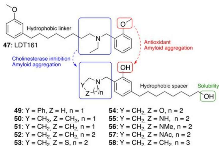
Figure 4. Cardanol-derived multifunctional compounds 49–58 .
