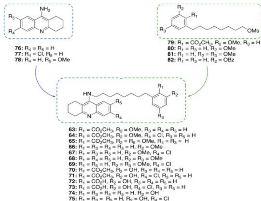
Figure 6. Design of CNSL-derived tacrine hybrid compounds 63–75 .
