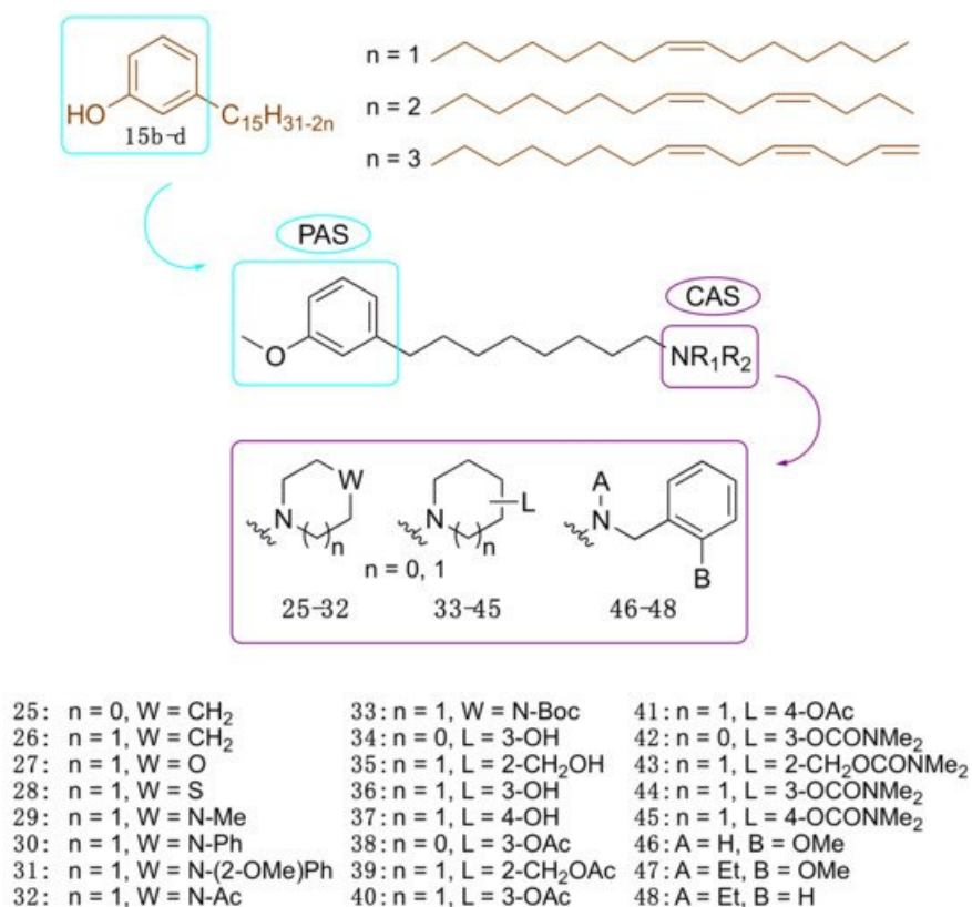
Figure 3. Cardanol-derived AChE inhibitors 25-48 .
