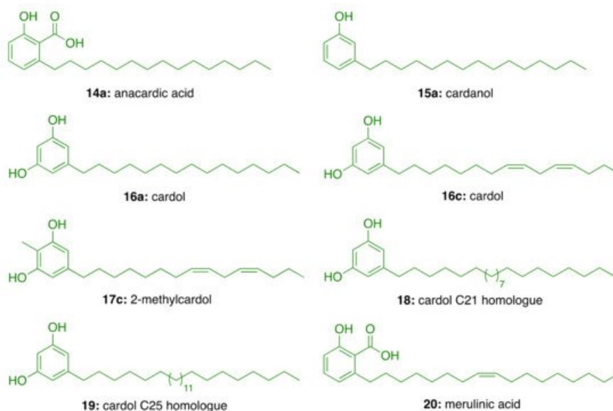
Figure 1. Phenolic lipids from A. occidentale , rye grain, and M. tremellosus .
