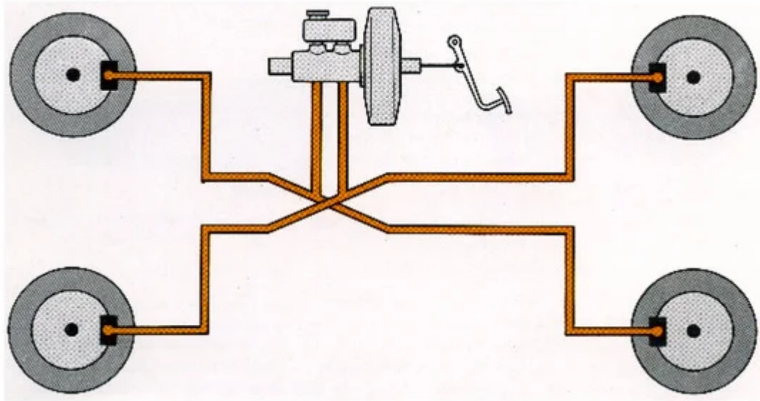
Figure 4. X-brake circuit.
