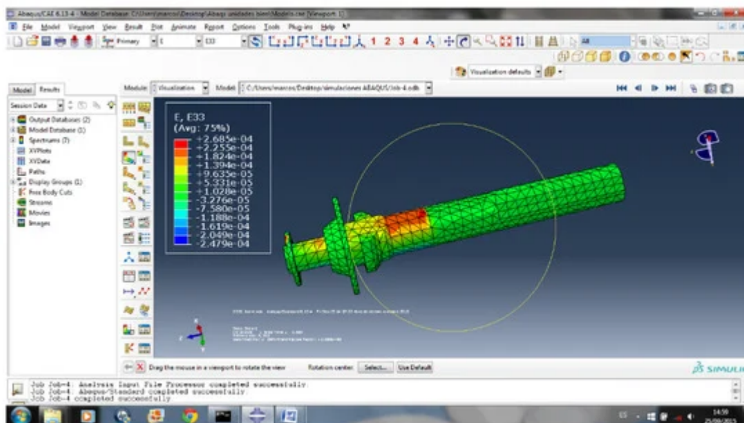
Figure 5. Results of the FEM simulation [Source: ABAQUS 6.13-4].
