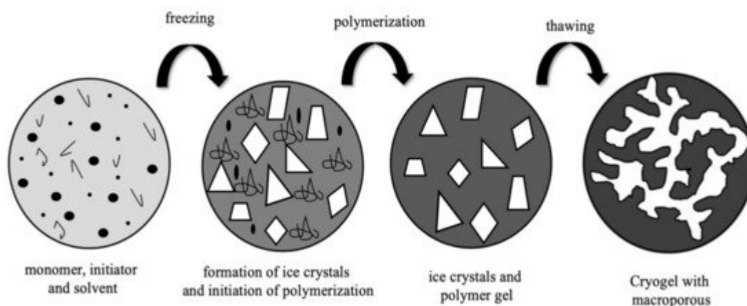
Figure 1. Illustration of supermacroporous cryogel preparation.
