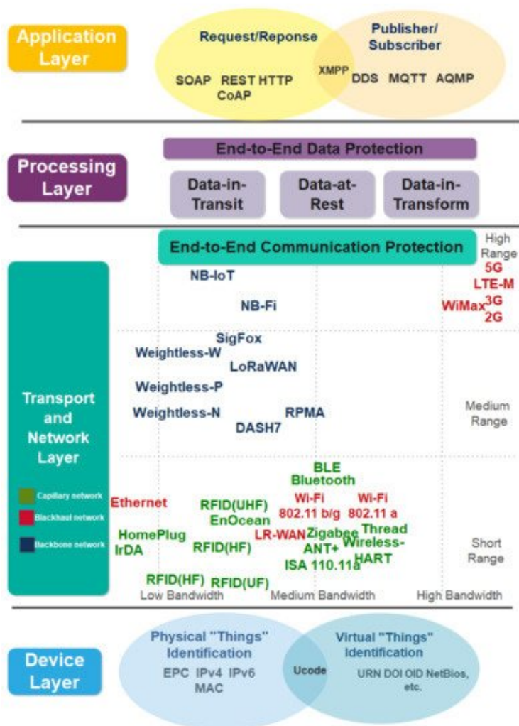
Figure 2. The proposed IIoT security architecture.
