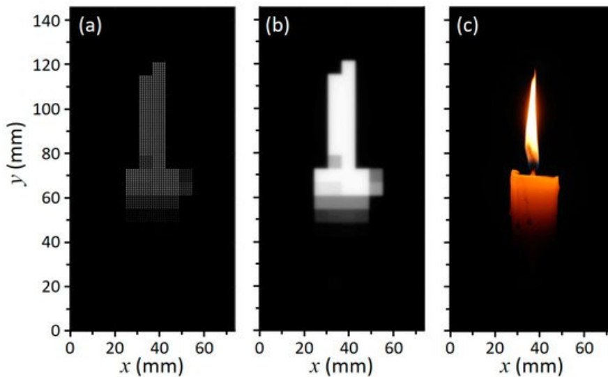
Figure 3. Displayed image simulation: (a) Mini-LED backlight modulation; (b) luminance distribution of the light incident on LC layer; and (c) displayed image after LCD modulation [18]. Figure reproduced with permission from Optical Society of America.
