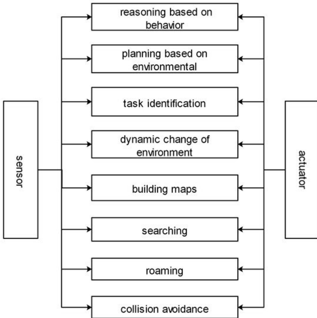
Figure 5. The behavior-based architecture.
