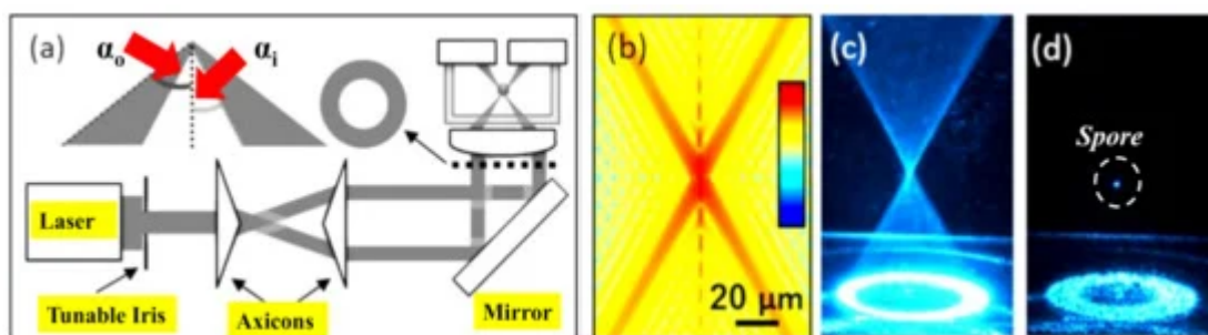
Figure 1. (a) Illustration of the optical trapping setup. The diameter of an expanded laser beam is managed with a tunable iris before travelling through the two axicons to form a collimated hollow beam. The aspheric lens creates a hollow conical focus within a glass chamber where airborne particles are trapped, adapted with permission from [43] . (b) Calculated intensity profile near the focal spot, adapted with permission from [43] . (c) Image of the conical focal region produced inside the chamber, adapted with permission from [43] . (d) Image of a spore captured in the air close to the focal point, adapted with permission from [43] .
