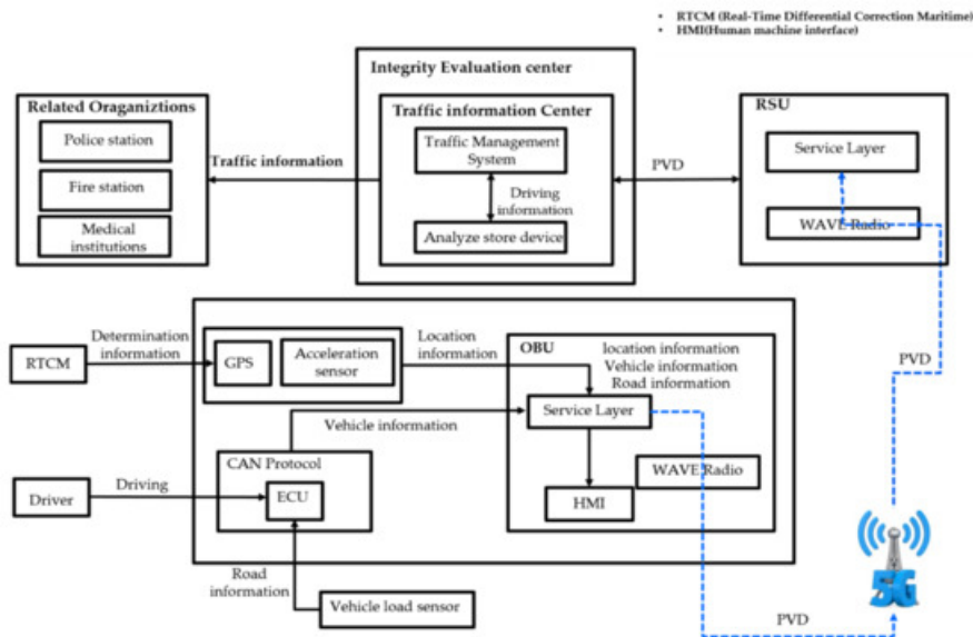
Figure 1. Location-Based Vehicle Data Collection Service.
