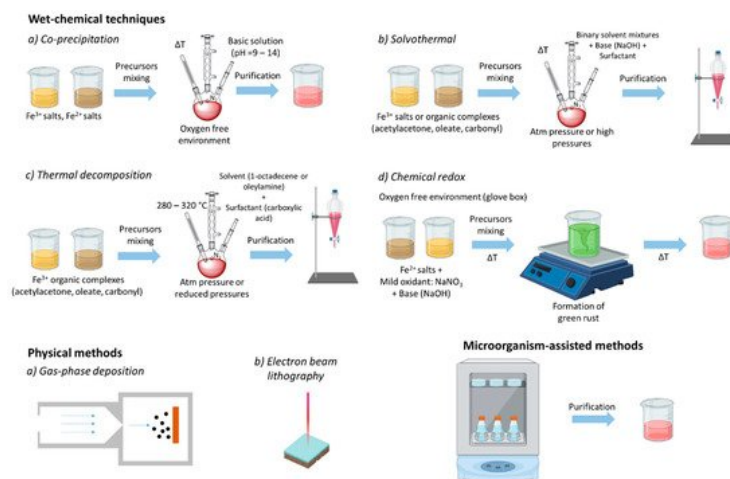
Figure 2. Different methods proposed for the synthesis of magnetic nanoparticles: wet chemical techniques (co-precipitation, solvothermal, thermal decomposition, chemical redox, etc.), physical methods (gas-phase deposition and electron beam lithography), and microorganism-assisted methods.
