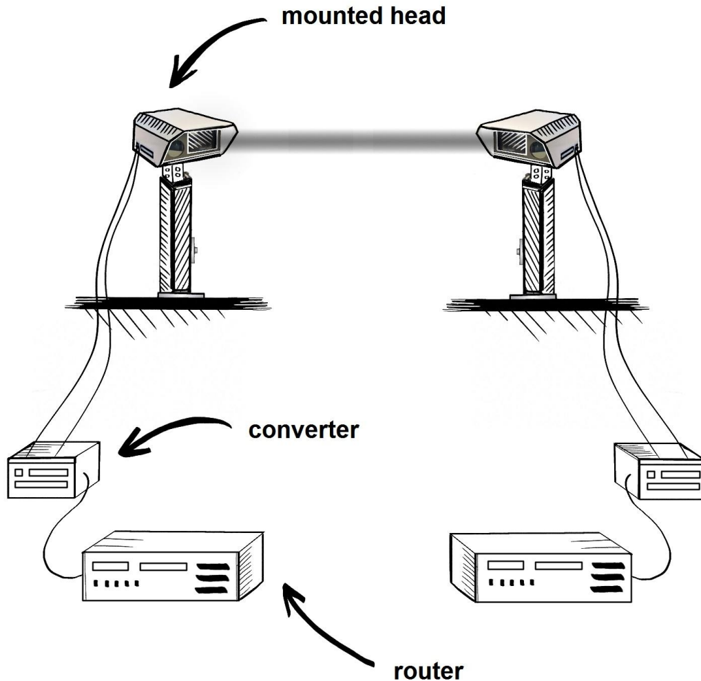
Figure 4. The scheme of the data transmission via Free Space Optics () technology between two heads.
