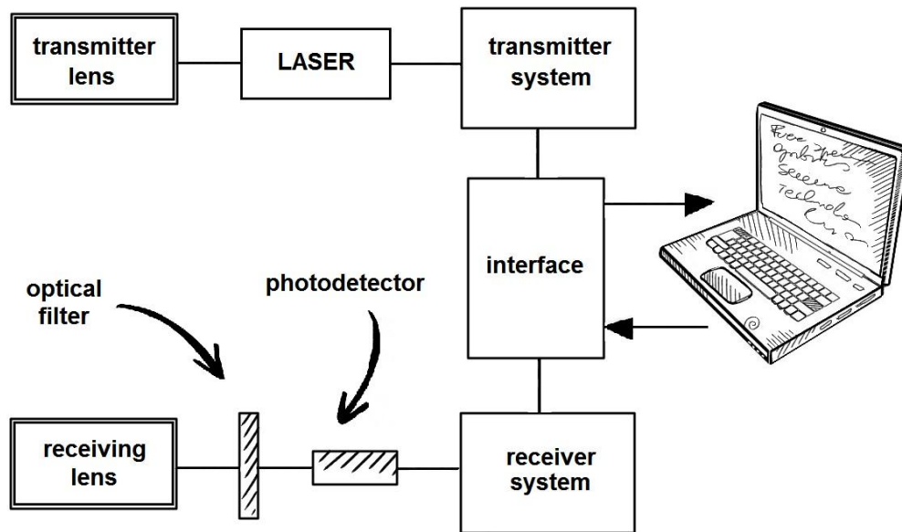
Figure 5. Block diagram of the FSO system.
