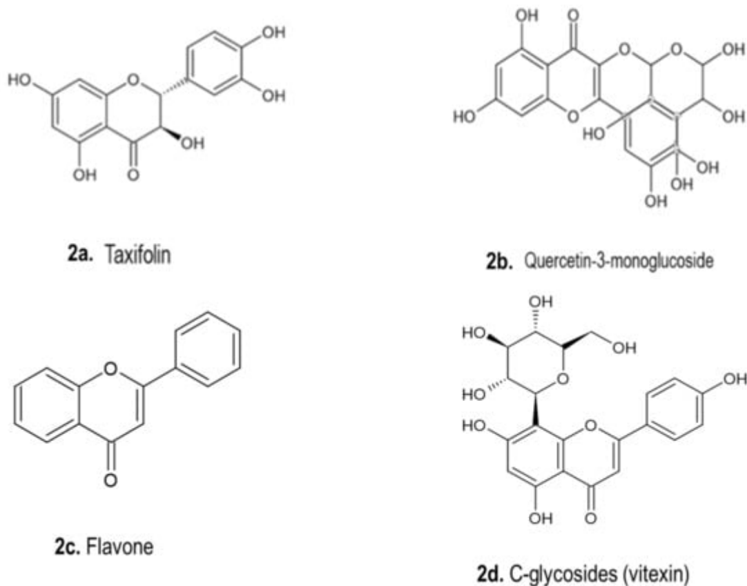
Figure 2. Chemical structures of phenolic compounds isolated from Drimia spp. [1]. (a). Taxifolin (Type of flavonoid, C_{15}H_{12}O_7 ); (b). Quercetin-3-monoglucoside ( C_{21}H_{19}O_{12} ); (c). Flavone ( C_{15}H_{10}O_2 ) and (d) Vitexin (Type of flavone glycosides, C_{21}H_{20}O_{10} ).
