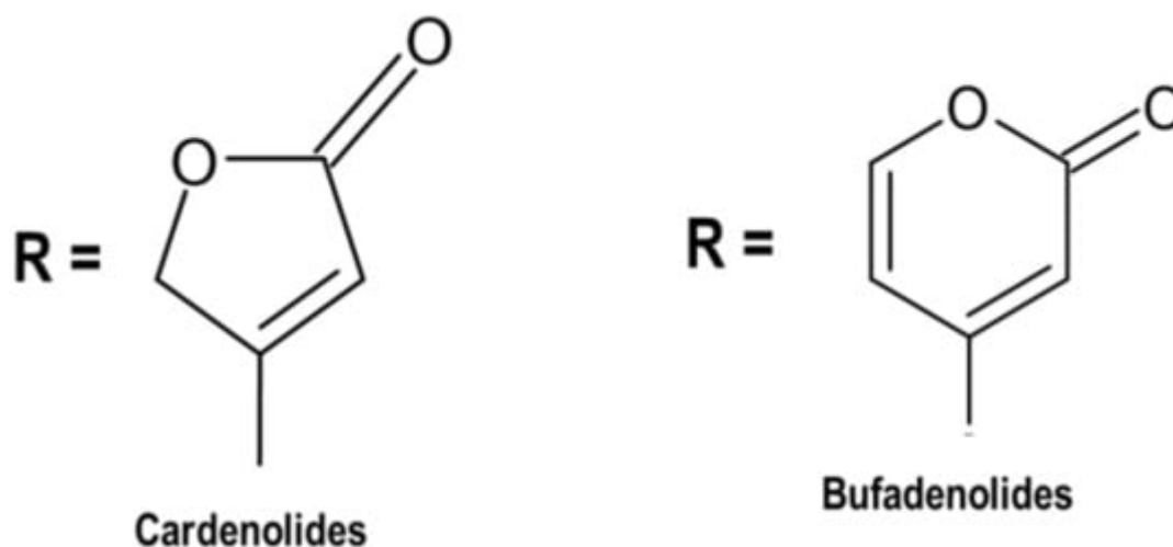
Figure 1. Two classes of cardiac glycosides occurring in nature [95].
