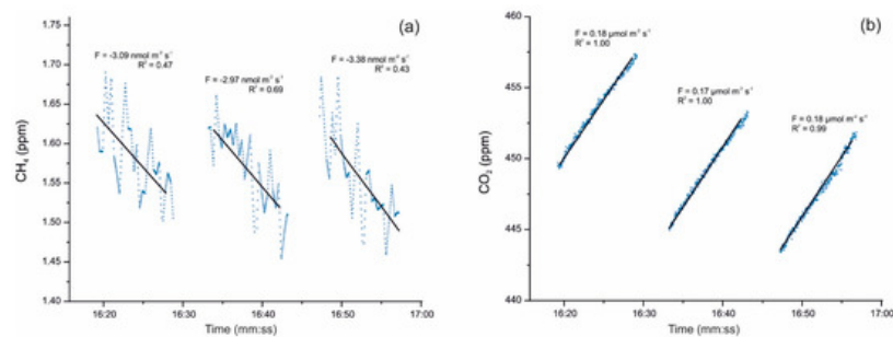
Figure 2. (a) Detail of CH 4 uptake fluxes with an average of -3.15 \text{ nmol m}^{-2} \text{ s}^{-1} and (b) simultaneous CO 2 emission fluxes uptake fluxes with an average of +0.17 \text{ μmol m}^{-2} \text{ s}^{-1} , monitored on 17 December 2019 directly above sediments inside Pindal Cave (Asturias, Spain). The value of the diffusive flux (F) and the corresponding exponential adjustment (R 2 ) of each measurement are indicated.
