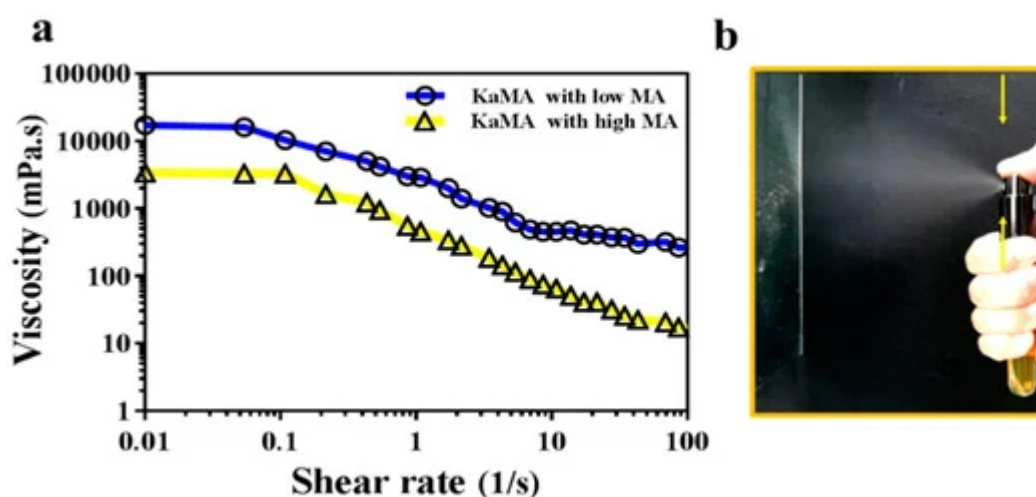
Figure 2. (a) Rheological evaluation of KaMA hydrogel with low and high MA degree; as shear rate increases, the viscosity drops; (b) spraying ability of the KaMA hydrogel with high MA [31].
