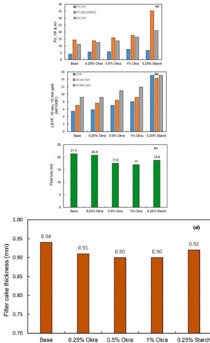
Figure 5. Graphical representation of okra powder as an eco-friendly additive in water-based drilling fluids. Increase in plastic viscosity, yield point, apparent viscosity, and gel strength (a,b), and decrease in fluid loss and mud cake thickness (c,d), using various additive concentrations (%) of okra powder versus starch [41].
