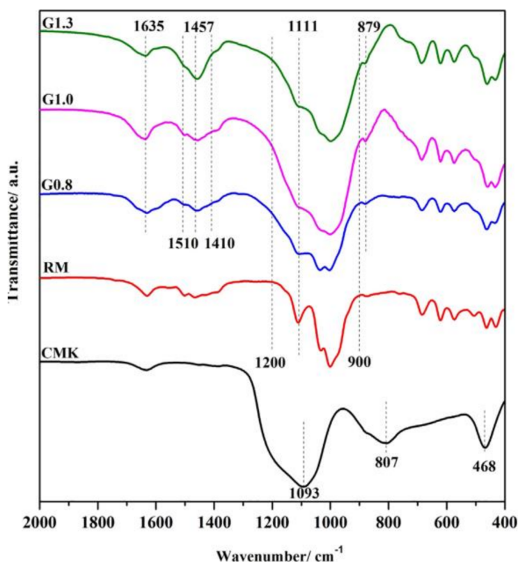
Figure 2. FTIR spectra of 28 d coal metakaolin
