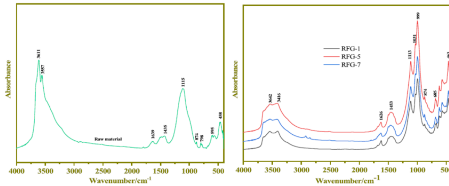
Figure 4. MIR spectra of mixed raw
