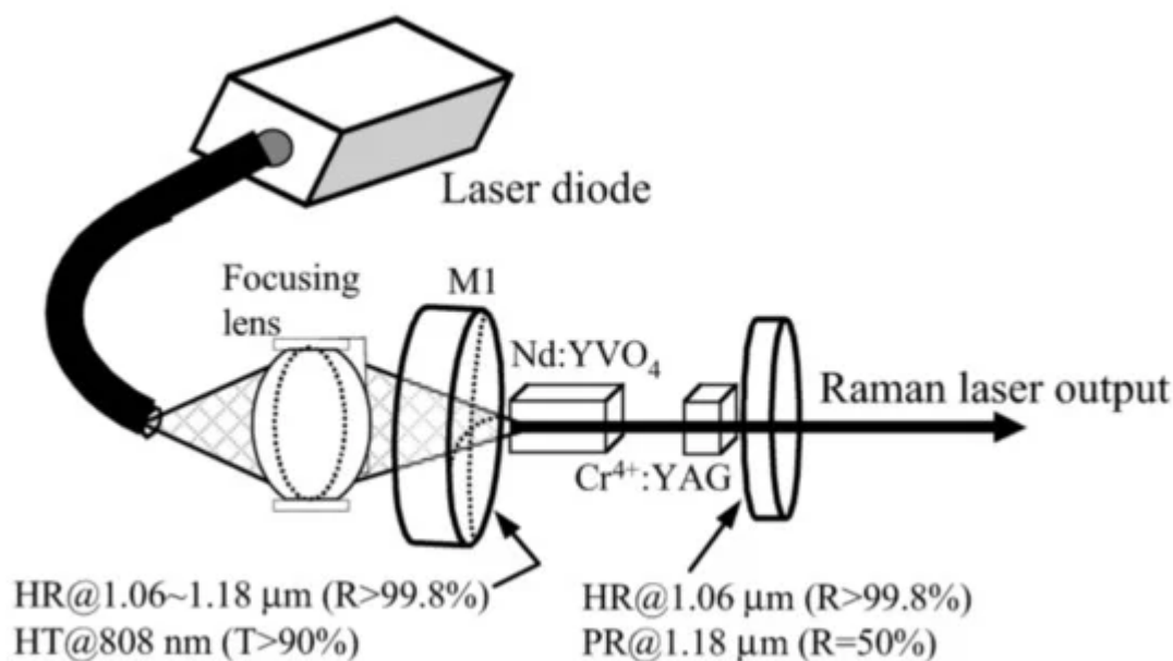
Figure 1. Schematic of the passively Q-switched \text{Nd:YVO}_4 self-Raman laser [23].
