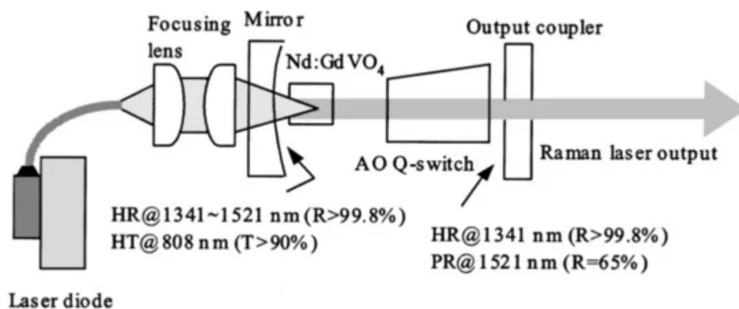
Figure 2. Schematic of actively Q-switched Nd:GdVO 4 self-Raman laser [18].
