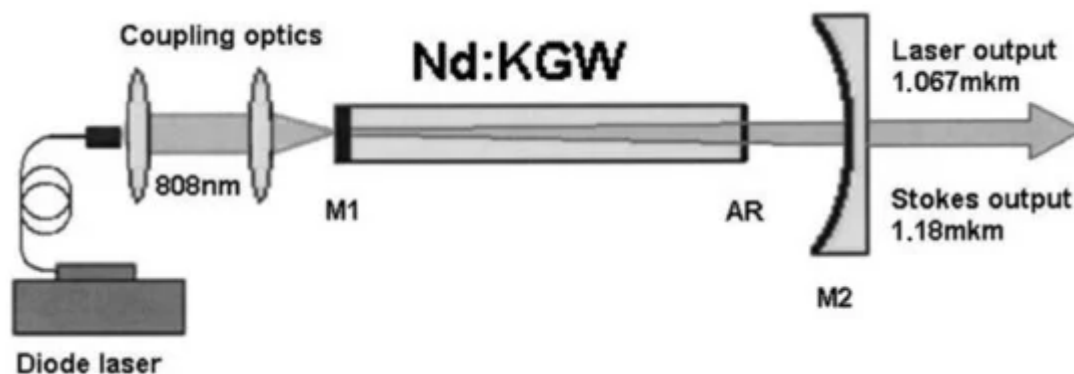
Figure 4. Schematic of the first continuous-wave self-Raman laser [2].
