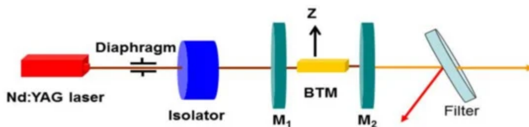
Figure 10. Schematic diagram of the BaTeMo 2 O 9 (BTM) self-frequency-doubled Raman laser at 589 nm [6].
