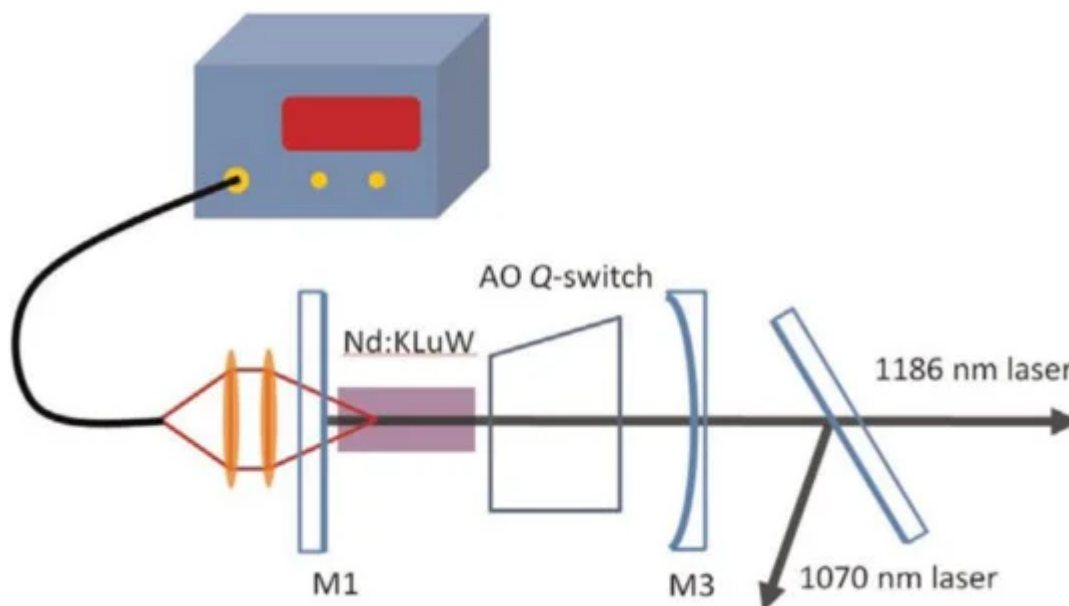
Figure 6. Schematic diagram of the actively Q-switched Yb:KLuW self-Raman laser [100].
