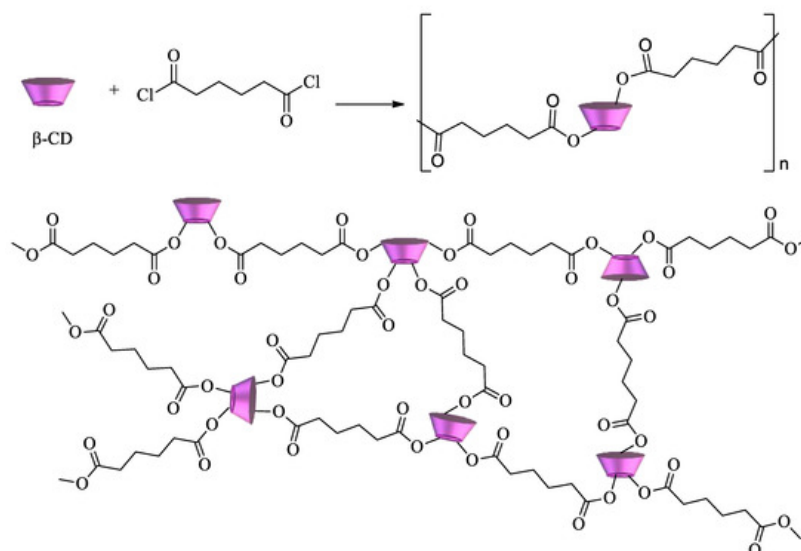
Scheme 3. β-CD polyester using adipoyl chloride as a crosslinking agent.
