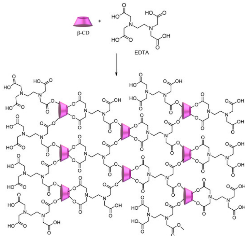
Scheme 4. CD–polycarboxylic polymer using ethylenediamine tetraacetic acid (EDTA) as a crosslinker.
