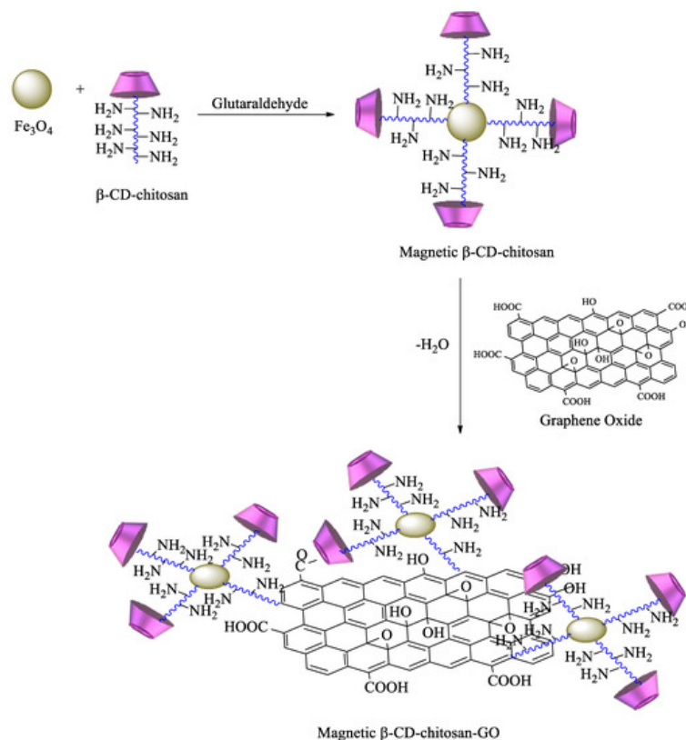
Scheme 7. Synthesis of magnetic \beta -CD–chitosan–graphene oxide (GO).
