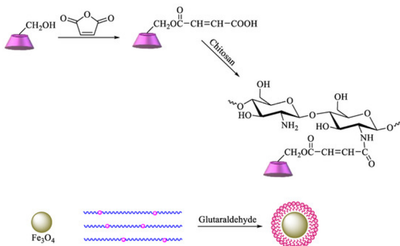
Scheme 6. Synthesis of \beta -CD–chitosan– \text{Fe}_3\text{O}_4 .
