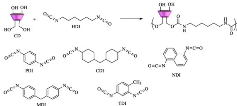
Scheme 2. Diisocyanates for the synthesis of CD-polyurethane copolymers.
