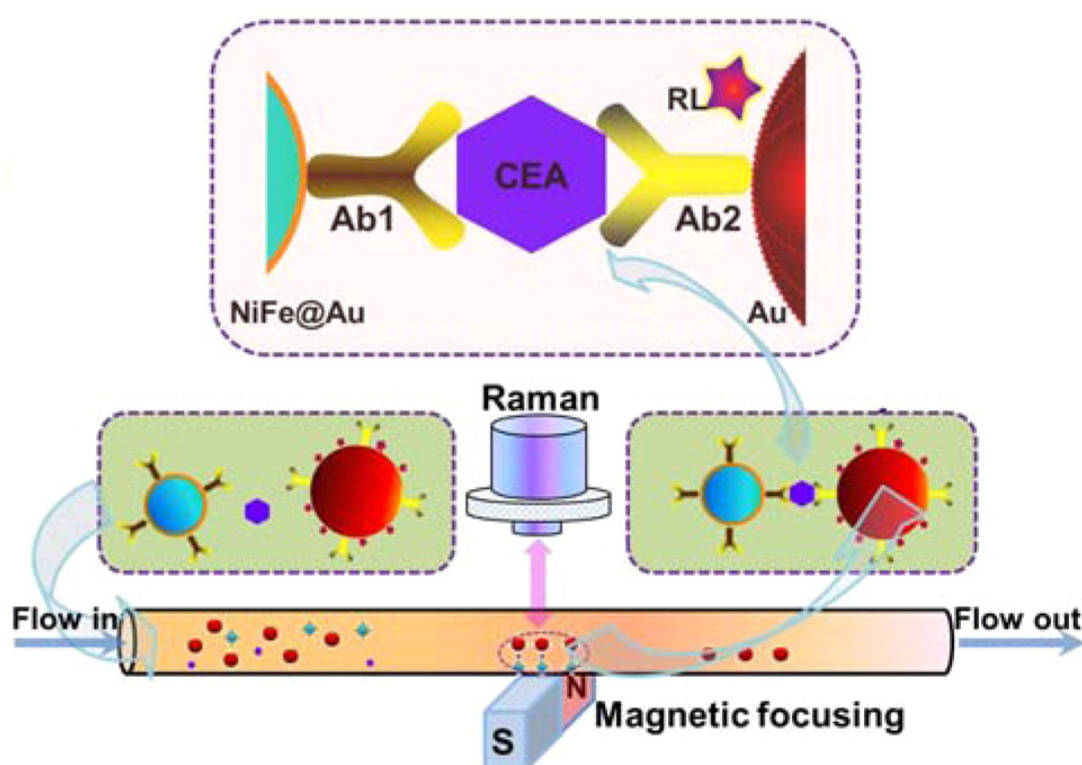
Figure 4. Illustration of SERS detection of cancer biomarker CEA (carcinoembryonic antigen). Using functional nanoprobe consisting of Au coated NiFe magnetic nanoparticles (NiFe@Au), capture antibodies (Ab1), detection antibodies (Ab2), and Raman labels (RL). Reprinted with permission from ref [101] . Copyright © 2015 American Chemical Society.
